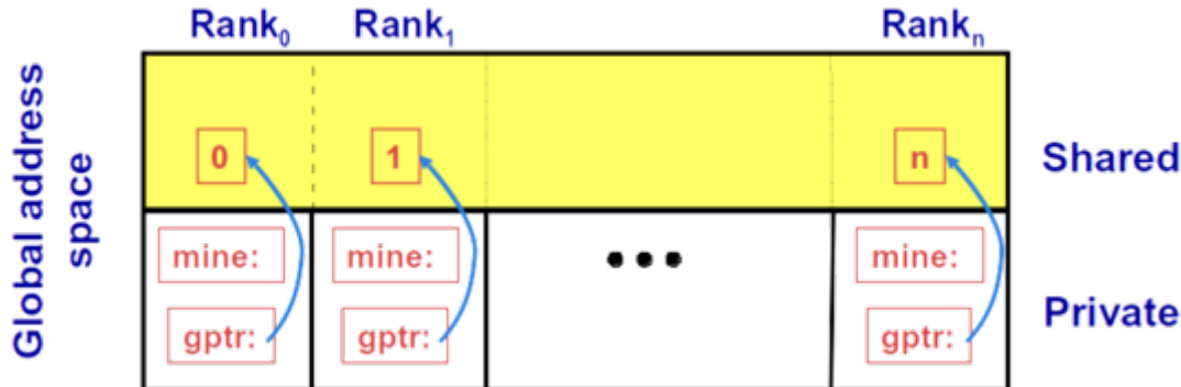
Figure 2: Global pointers.
