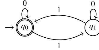
Figure 3: Finite automaton checking whether the number of “1”s is even.
