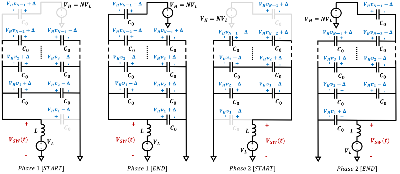
Figure 5. Phase progression for the generalized 1:N D-IL-direct converter undergoing step-up split-phase operation with all flying capacitors set equal. Circuit configurations and flying capacitor voltages (left and right side symmetric) are depicted for both the start and end of each phase.
