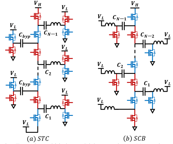
Figure 2. Example multi-inductor Dickson variants: (a) one instantiation of the switched tank converter (STC) [43], (b) series-capacitor buck (SCB) converter [54]–[56]. Assuming appropriate passive values, both the depicted STC and SCB may be simplified into the S-1L-tank-alt (Fig. 1 (d)) and S-2L-direct_PWM (Fig. 1 (g)) respectively by consolidating switches and lumping passive elements.
