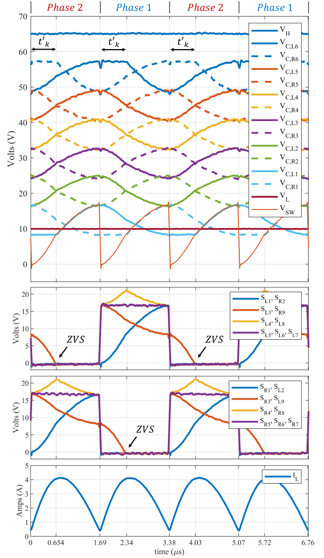
Figure 9. Measured voltage and current waveforms of a 1:7 resonant instantiation of the D-1L-direct split-phase Dickson variant analyzed in Section VI. With V_L = 10 \text{ V} , these results validate the derivation of (63), (64), (65), and (66).
