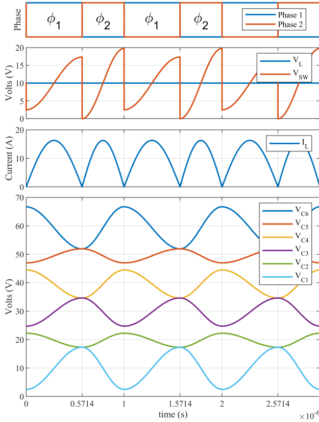
Figure 4. Simulated LTSpice waveforms of a 2-Phase 1:7 S-1L-direct converter operating with maximum allowable charge conduction, q_{H,max} . Phase 2 ( \phi_2 ) commences with V_{SW} = 0V , signifying that a further load increase would result in unintended reverse conduction in switches S_2 and S_3 .
