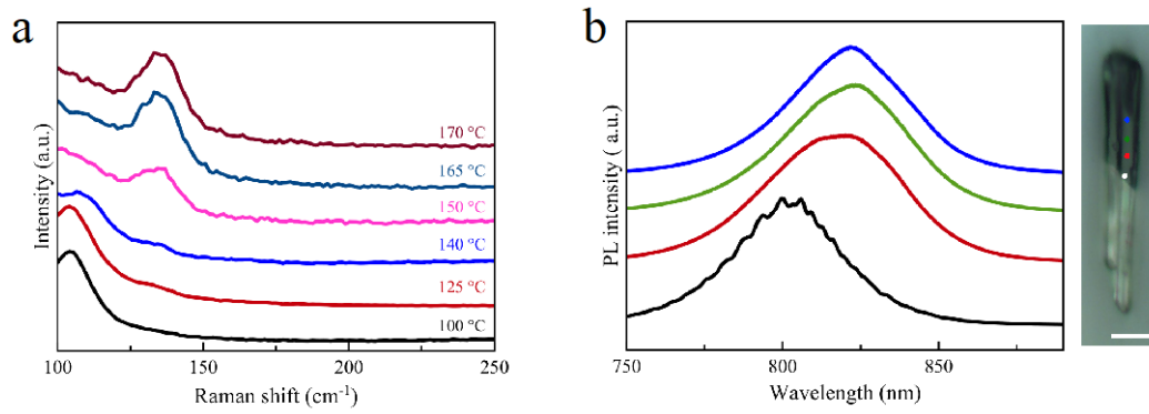
Figure 2. Optical measurements of FAPbI 3 phase transition. (a) in-situ Raman spectra evolution from low-T phase to high-T phase FAPbI 3 . (b) Confocal PL spectra of a low-T/high-T two-phase heterojunction. The PL spectra of blue, green, red, black are corresponded to PL emission of the spots (blue, green, red, white) in the optical image. The scale bar is 5 μm.
