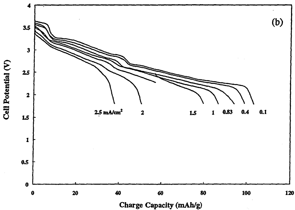
Figure 4-18. Discharge curves for Na/PEO n NaCF 3 SO 3 /Na x CoO 2 , where (a) n = 8, and (b) n = 20.
