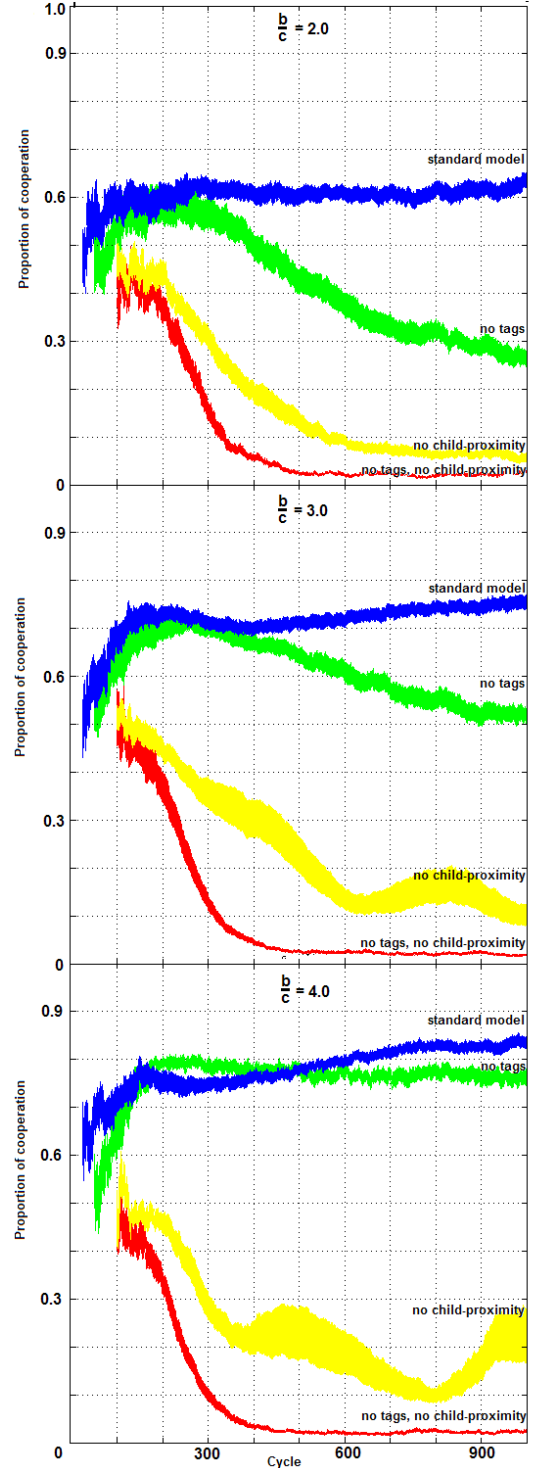
Figure 1: Proportion of cooperative interactions averaged over 30 simulations vs. cycle for the standard model and three simplified conditions with 3 different b/c ratios. Line thickness indicates 1 SE around the mean. The data start at cycle 25 for the standard model (blue), cycle 50 for no tags (green) and cycle 100 for no child proximity (yellow) and no tags or child proximity (red). Data before the start cycle were omitted for clarity because their SEs were too high to be meaningful.
