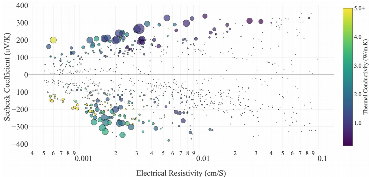
Figure 0. Thermoelectric properties of nearly 1000 materials compiled by Gaultois et al. [86] and as retrieved and visualized with matminer. The marker size is scaled according to the figure of merit, zT .
