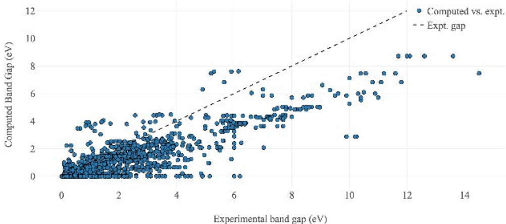
Figure 0. Comparison of experimentally-measured band gap energies retrieved from the Citrine database to DFT-PBE computed electronic band gaps retrieved from the Materials Project. As expected, the data set demonstrates that computed band gaps underestimate experimental values.[87–89]
