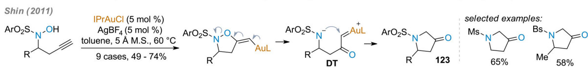
Scheme 65. Synthesis of 3-Pyrrolidinones via Gold-Catalyzed Alkyne Oxidation with N -Sulfonyl Hydroxylamines
