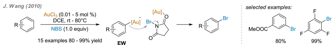
Scheme 77. Gold-Catalyzed Bromination of Aromatic Rings
