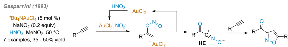
Scheme 105. Gold-Catalyzed One-Pot Synthesis of Isoxazoles from Terminal Alkynes and Nitric Acid
