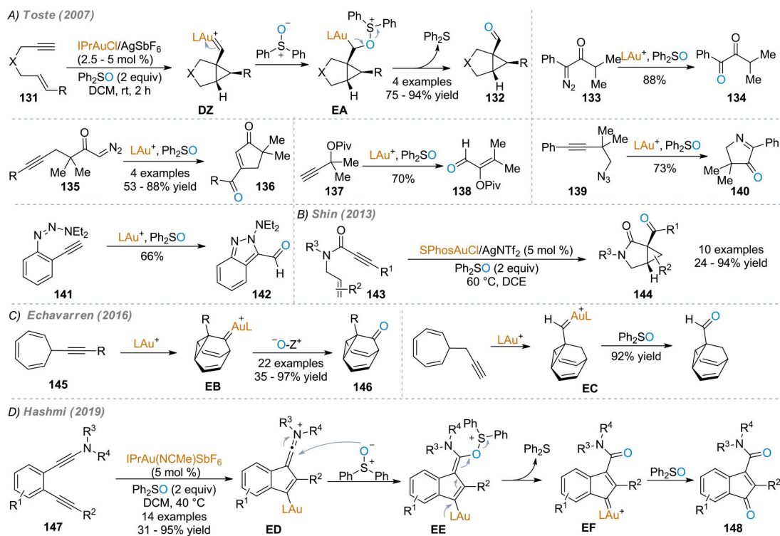
Scheme 69. Oxidation of Gold Carbene by Sulfoxides
