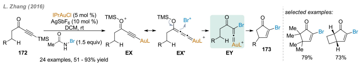
Scheme 78. Gold(I)-Catalyzed C–H Insertion Reaction by In Situ -Generated Gold Vinylidenes
