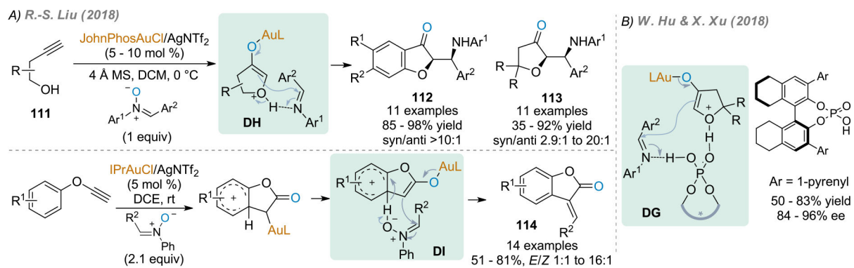
Scheme 60. Gold-Catalyzed Alkyne Oxidation by Nitrones Terminated by the Mannich Reaction
