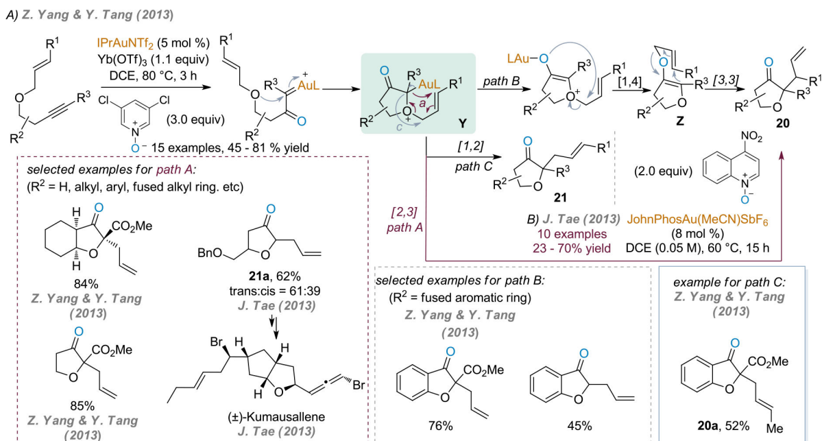
Scheme 11. Rearrangements of Oxidatively Generated Allyl Oxonium Ions
