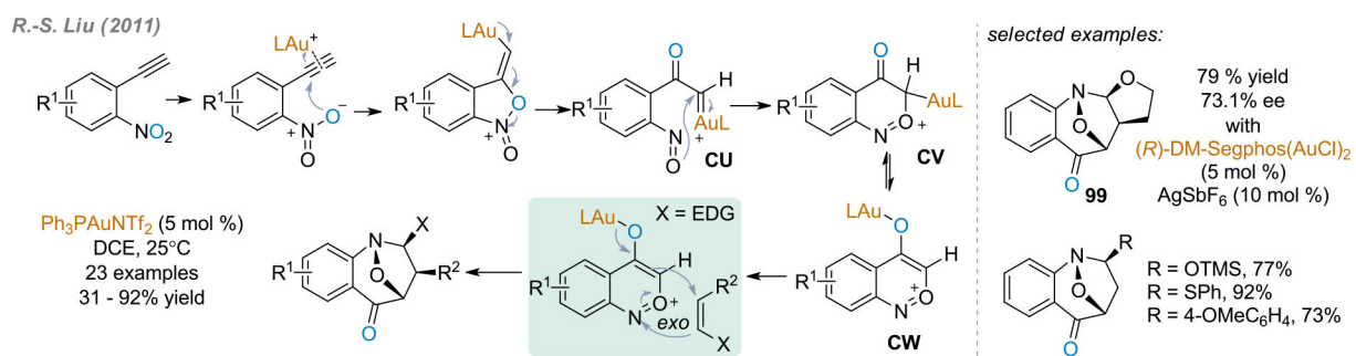
Scheme 55. Gold-Catalyzed Oxidative Cycloaddition Cascade of o -Nitrophenylacetylenes
