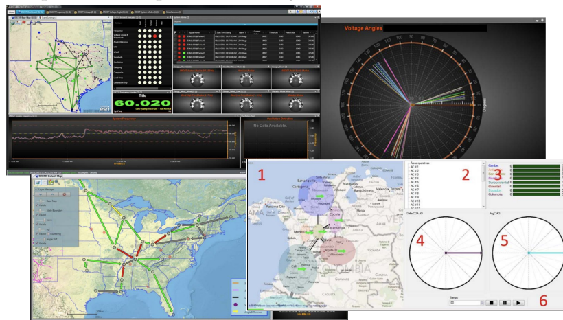
Figure 15: Interfaces of industry tools for angle difference monitoring. Clockwise from top left: ERCOT, Dominion, Columbia WAMS, and EPG [100]
