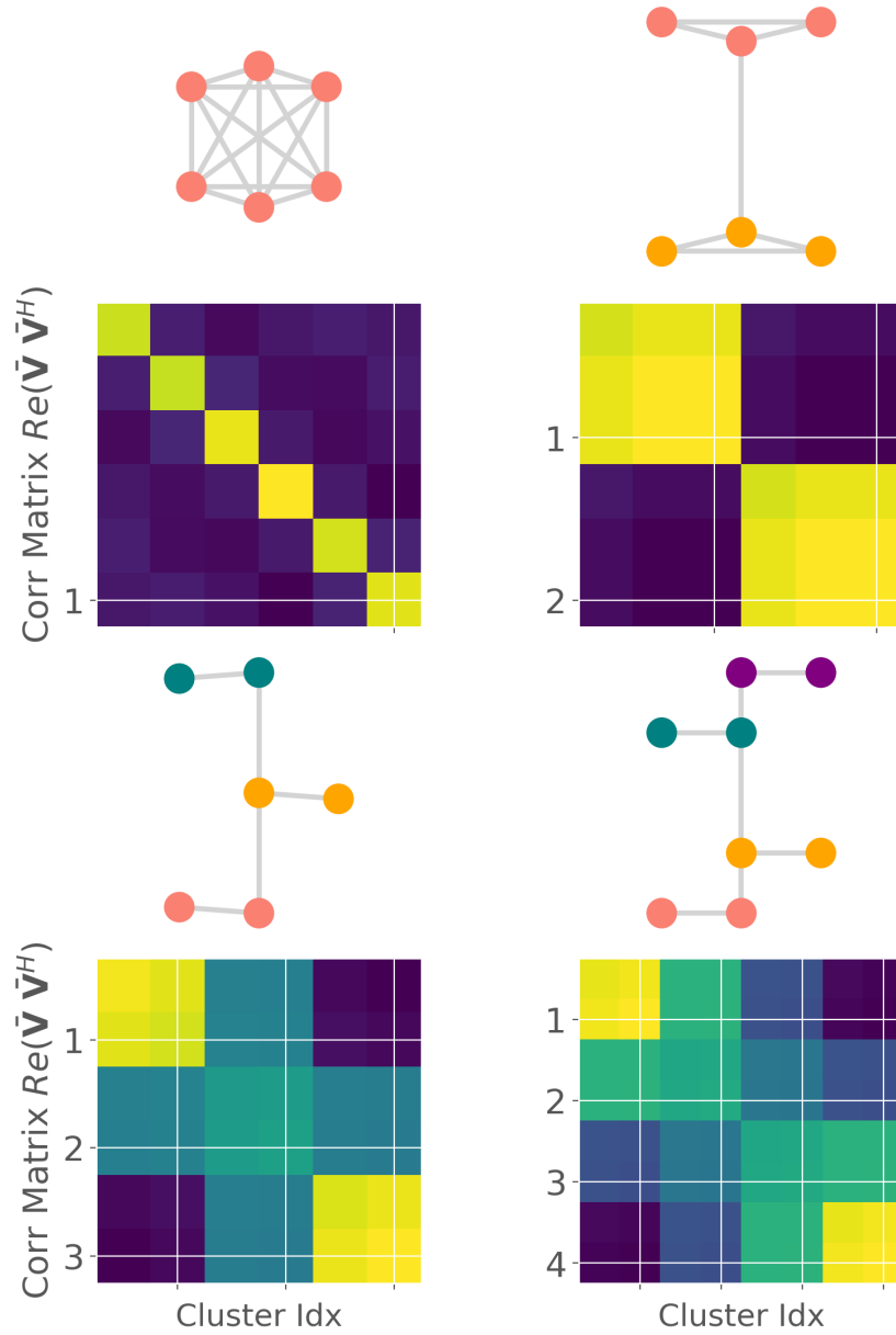
Figure 44: Results of node clustering by clustering voltage correlation matrix \mathcal{S}^{(V)} = \bar{V}\bar{V}^H with k-means. Node color indicates cluster membership. Plots show \text{Re}(\mathcal{S}^{(V)}) for each network.
