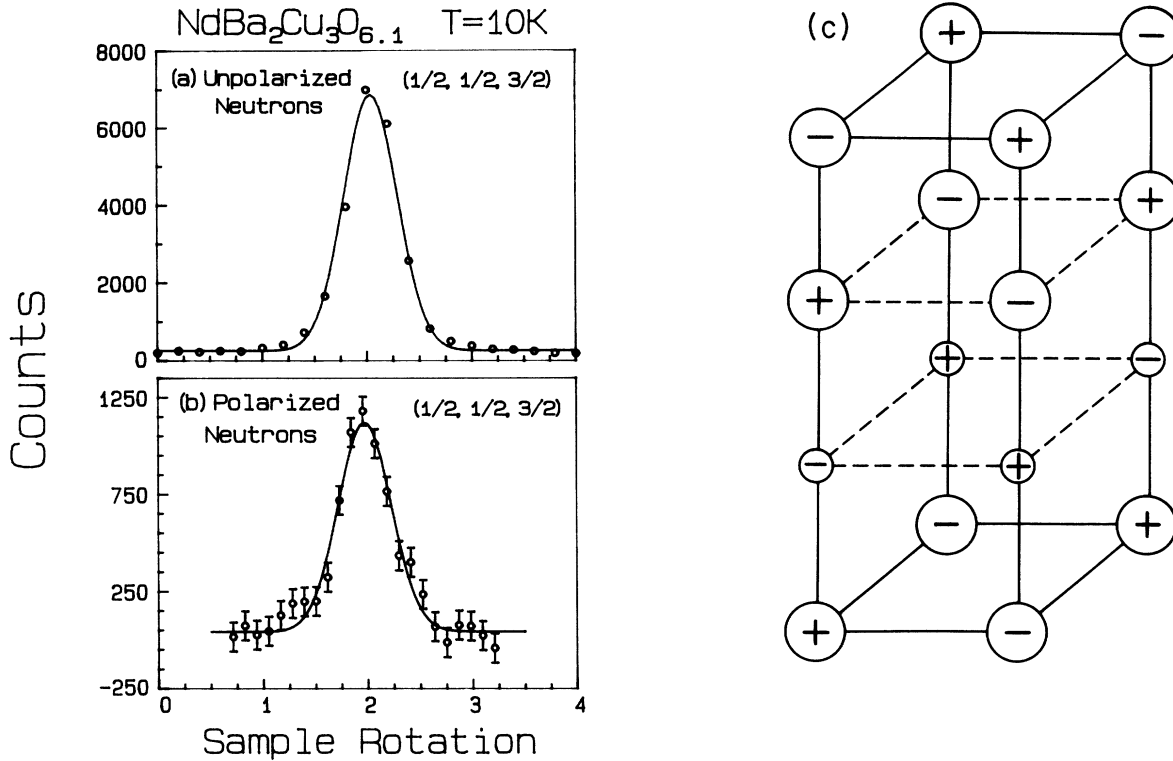
FIG. 3. The (\frac{1}{2}, \frac{1}{2}, \frac{3}{2}) Bragg reflection from the x=0.1 crystal at T=10\text{ K} is shown. (a) The unpolarized beam result. (b) The polarized beam result, where the difference of the observed intensities between the \mathbf{B}\parallel\mathbf{Q} and \mathbf{B}\perp\mathbf{Q} configurations is plotted. The data demonstrate that the scattering is magnetic in origin. The solid curves are a least-squares fit to a Gaussian (resolution) function. (c) The basic spin structure for the Cu moments at low T . There is a substantial moment on the Cu ions in the oxygen deficient chain layer (small circles).
