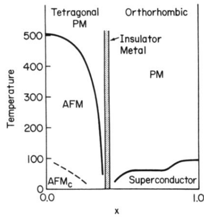
FIG. 2. Schematic phase diagram for \text{RBa}_2\text{Cu}_3\text{O}_{6+x} as a function of oxygen concentration x on the chain sites. There are two antiferromagnetic phases in the small x regime: AFM, in which only the Cu spins in the plane layers are ordered, and \text{AFM}_C , in which the Cu spins in the chain layers are also ordered. At large x or at very high temperatures the Cu ions are paramagnetic (PM).
