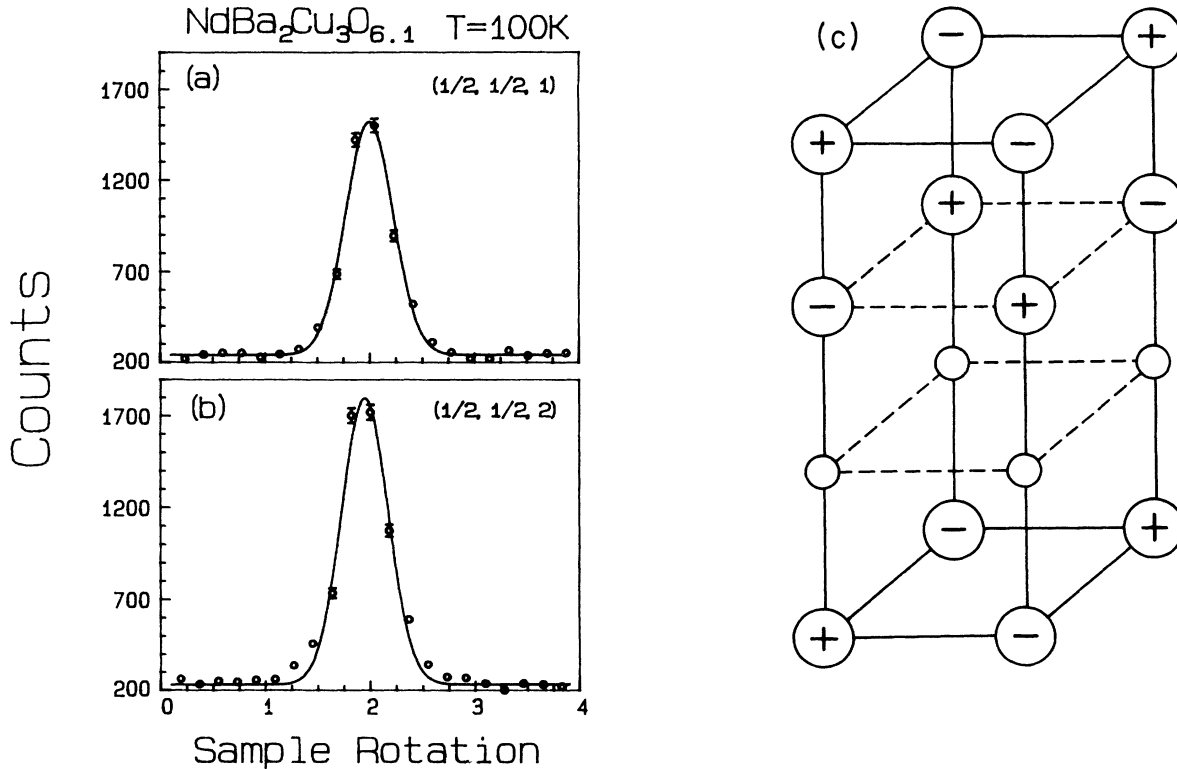
FIG. 4. Two typical magnetic Bragg reflections in the high- T phase. Shown are the (\frac{1}{2}, \frac{1}{2}, 1) and (\frac{1}{2}, \frac{1}{2}, 2) reflections from the x=0.1 crystal at T=100 K. The basic spin structure for the Cu moment at high T is shown in (c). The Cu moments in the oxygen-deficient planes (small circles) are thermally disordered.
