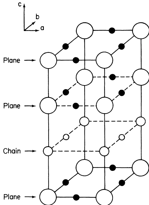
FIG. 1. The crystal structure of \bar{R}\text{Ba}_2\text{Cu}_3\text{O}_7 , with only the Cu (open circles) and O ions (solid and shaded circles) in the copper-oxygen layers indicated for clarity. The rare-earth ion is located between the two plane layers, while the plane and the chain layers are separated by a BaO layer. The occupancy of the oxygen sites in the chain layer (shaded circles) can be readily varied from full occupancy ( x=1 ) to full depletion ( x=0 ).
