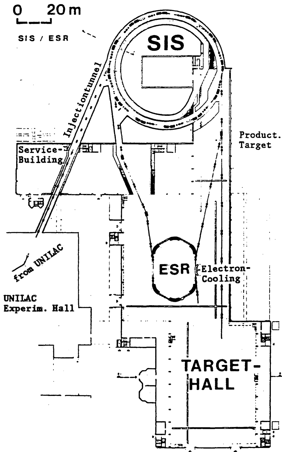
Fig. 5. The GSI SIS-18 heavy ion synchrotron and ESR storage ring, under construction 11 . XBL 8611-4587
