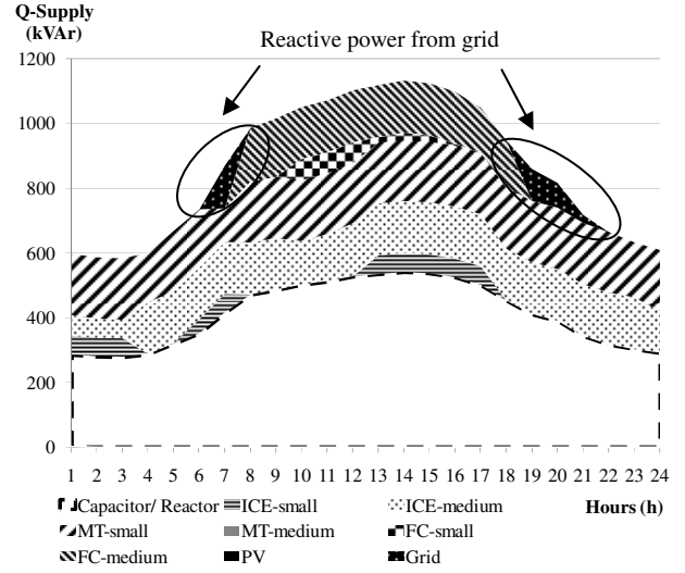
Fig. 5: Reactive power supply for scenario 2 with enabled grid procurement for the month of June
