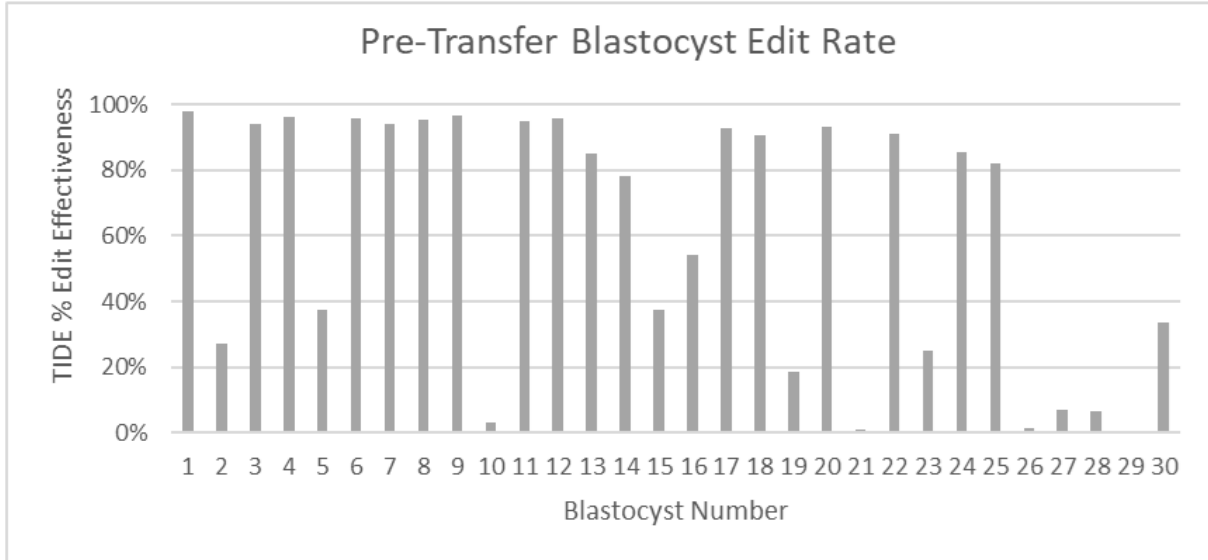
Figure 7: Bar chart demonstrating TIDE analysis estimated percent edited based off Sanger sequencing data of blastocysts created prior to transfer embryo creation date with guide A and embryo round 1 and 2 primers.
