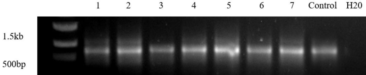
Figure 3: Gel product demonstrating all 7 sheep DNA band alignments to the control band of the expected size.
