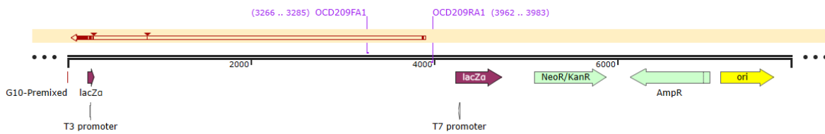
Figure 8: SnapGene alignment demonstrating the aligned sequence with a large unaligned insertion.
