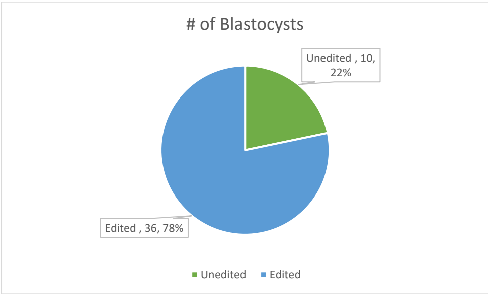
Figure 2. Pie chart demonstrating the percentage of blastocysts not transferred that contained edits compared to unedited blastocysts.
