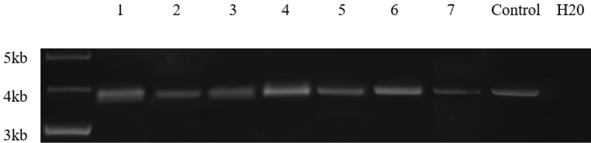
Figure 5: Edited sheep and control bands from the long PCR (3825bp) showing similar band length to control.
