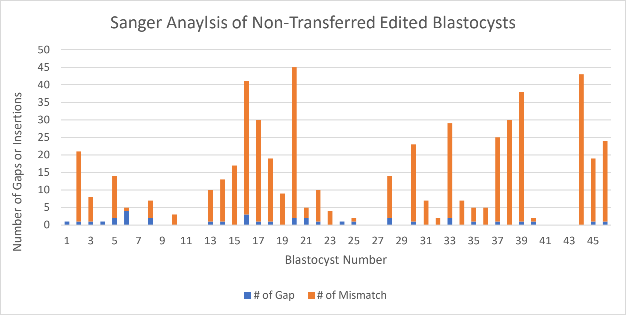
Figure 1: Blastocysts identified with their number of gaps (insertions or deletions) and/or base pair mismatches when aligned to an un-edited reference genome.
