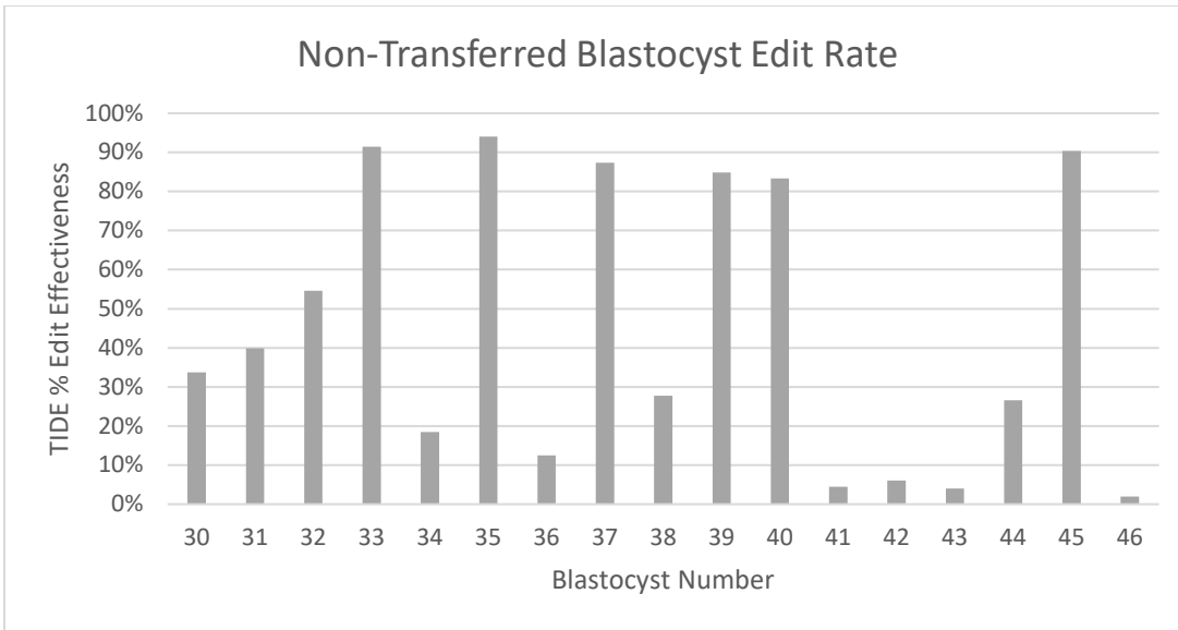
Figure 6: Bar chart showing the TIDE analysis estimated percent edited based off Sanger sequencing data of blastocysts created for transfer that were not transferred.
