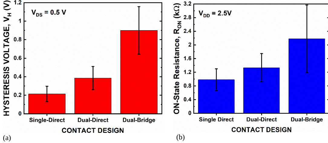
(a) (b) Fig. 4.3 Average measured values of (a) V_H and (b) R_{ON} for 10 relays of each contact design with V_B = 0 V. The bars indicate the ranges of standard deviation.
