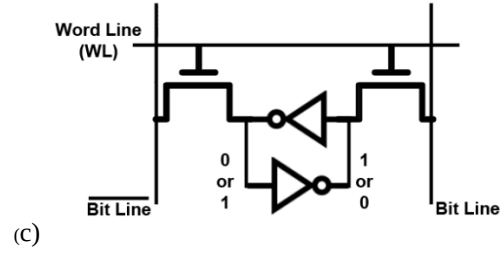
DRAM cell
