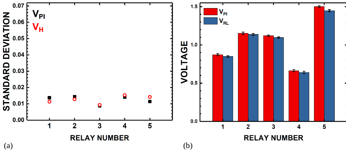
Fig. 3.8 Measured (a) variability in V_{PI} , V_H and (b) switching voltages for multiple PFOTES relays operated at V_{DS} = 1 V, V_B = -16 V. L = 8 \mu m.
