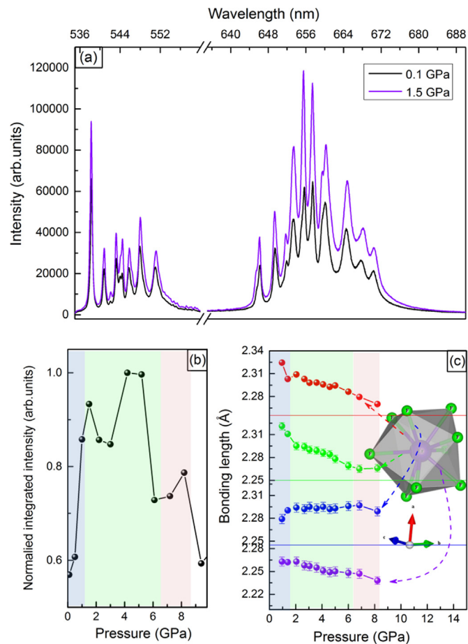
Fig. 5. (a) Comparison of fluorescence intensity at 0.1 GPa and 1.5 GPa. (b) Fluorescence intensity as a function of applied pressure and (c) Pressure dependences of the length of Er-F bonding of \text{ErF}_3 .
