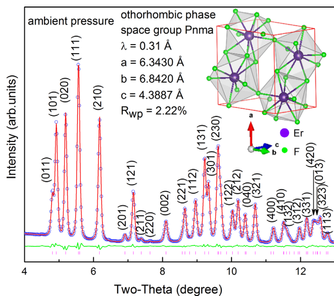
Fig. 1. The XRD pattern of \text{ErF}_3 under ambient conditions. The inset is the schematic crystal structure of \text{ErF}_3 .
