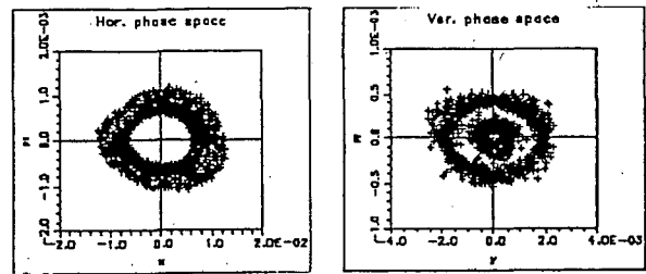
Figure 4. Phase space at injection.
