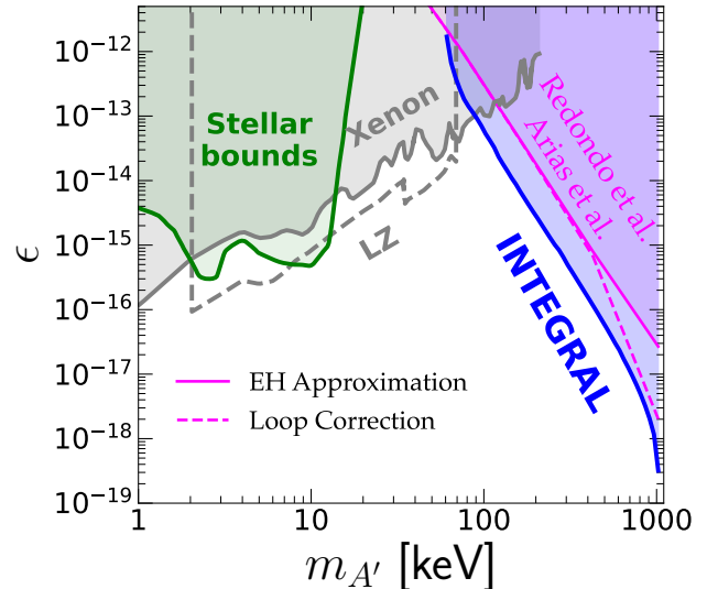
FIG. 4. New constraints on the plane of the kinetic mixing and the dark photon mass using INTEGRAL/SPI are shown in blue. Previous constraints based on this decay process based on the diffuse X-ray background is in magenta: solid line is the leading EFT result [8–10], and the dashed line includes the full one-loop decay amplitude. Constraints on dark photon from direct searches are shown in gray: the solid line is from Xenon and the dashed line the projection for LZ [11–15]. The combined constraints from studies of dark photon production in stars (stellar bounds) are in green and follow the results of Refs. [16–18, 20–26].
