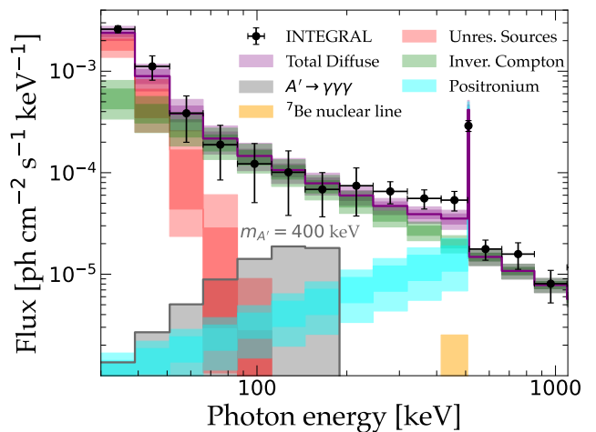
FIG. 3. The INTEGRAL photon flux and models for different sources. The observed data between 30–1022 keV are shown as black points. The best fit, along with 1\sigma and 2\sigma error bands for the astrophysical source classes are depicted as follows: Red for Unresolved Sources, green for Inverse Compton scattering, Positronium decay with an intensity fit to the 511 keV line is shown in cyan, and ^7\text{Be} nuclear line is in orange. The Total Diffuse Flux that fits the data is in purple. For comparison, we also show an arbitrarily normalized spectrum for the dark photon trident from a 400 keV dark photon (gray band), which is not included in the fit.
