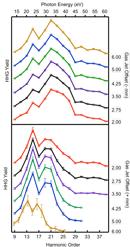
Figure 3: Intensity dependence of the measured SF 6 harmonic spectrum at (-) and (+) 2.75 mm.
