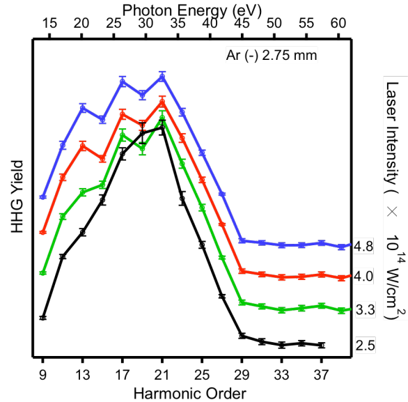
Figure 4. Intensity dependence of the measured Ar harmonic spectrum at (-) 2.75 mm.
