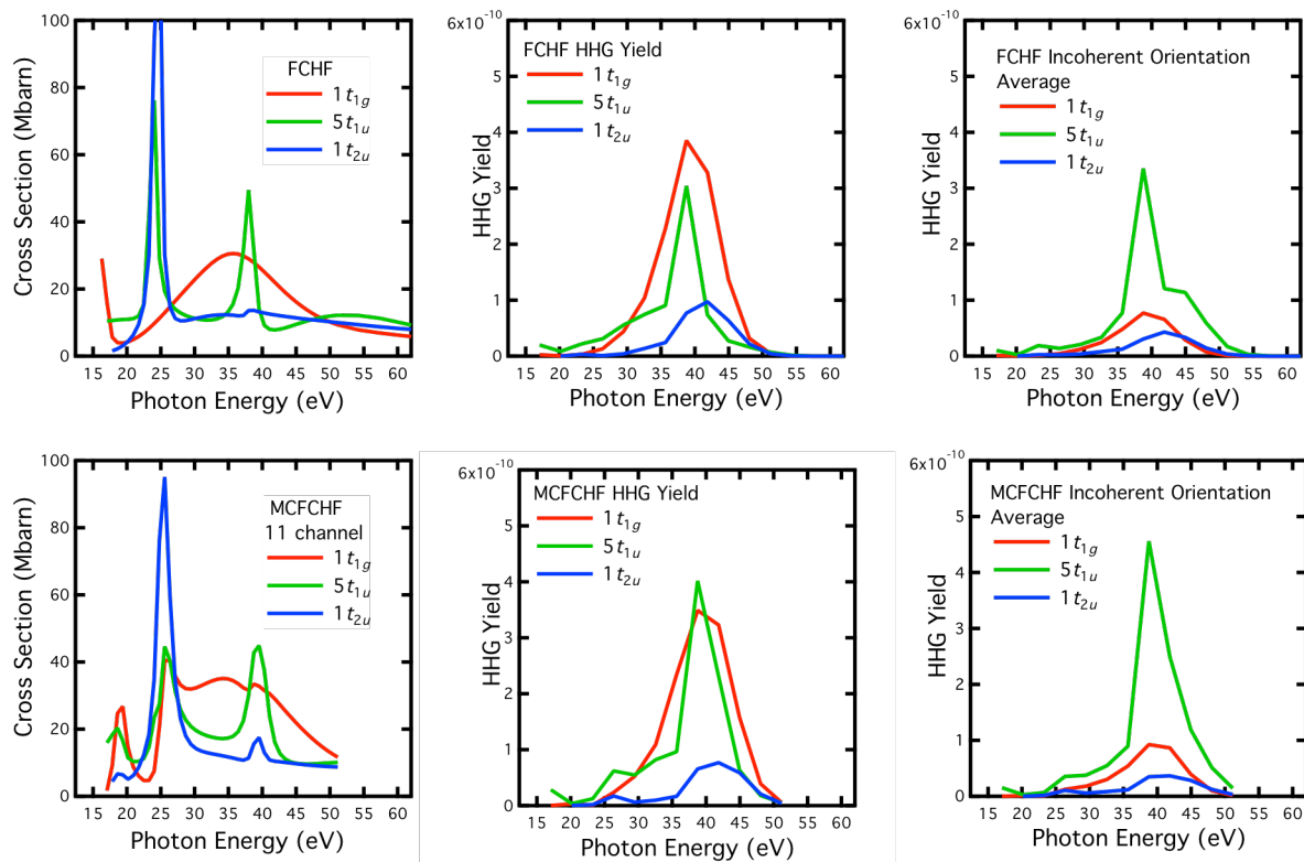
Figure 6. Photoionization cross sections and QRS HHG spectra of \text{SF}_6 for the outer three valence orbitals, 1t_{1g} (HOMO), 5t_{1u} (HOMO-1), and 1t_{2u} (HOMO-2). Left column is the computed photoionization cross sections. Center column is the QRS HHG spectra from the different channel terms in Eq. (8), which has a coherent orientation average. Right column is the approximate separate-channel HHG spectra obtained from incoherent orientation average given in Eq. (9). The top row contains the results for the single-channel FCHF calculations and the bottom row has the corresponding data from the coupled channel MCFCHF calculations.
