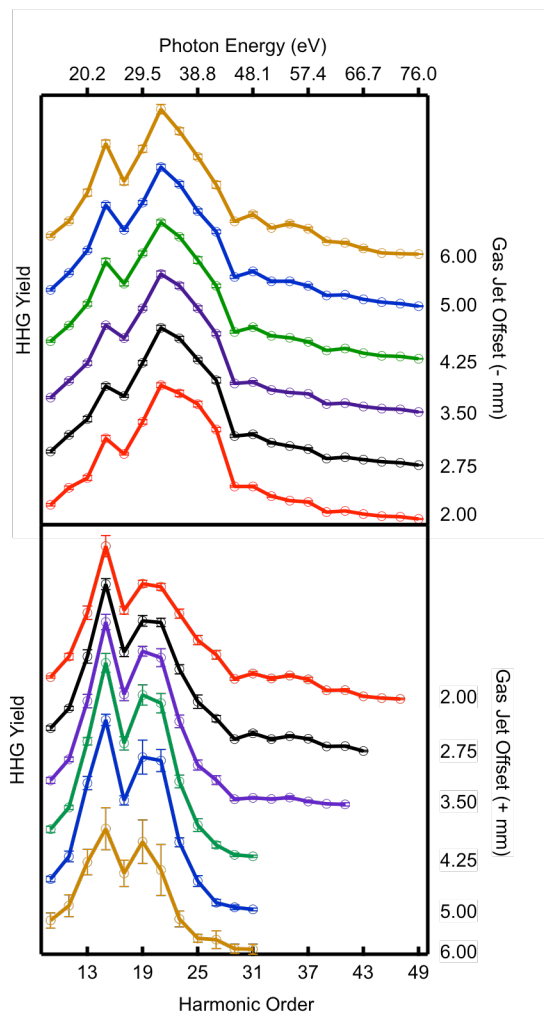
Figure 2: Position dependence of the measured SF 6 harmonic spectrum at 4.0 \times 10^{14} W/cm 2 . The (-) positions indicate a situation where the focal point is in front of the center of the gas jet.
