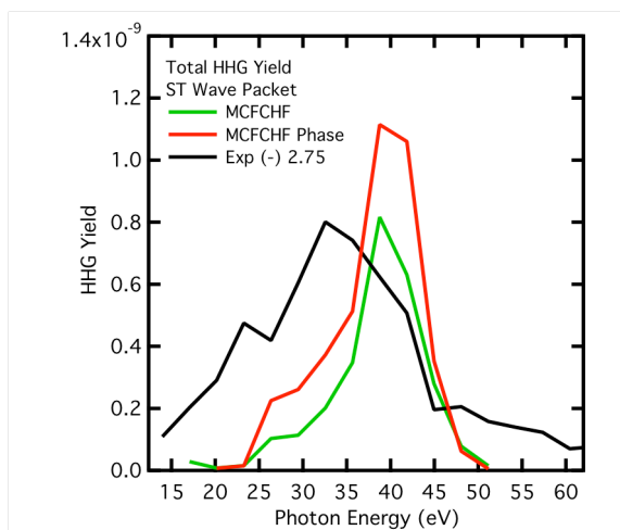
Figure 9. Comparison of HHG yield computed from the incoherent sum from the different channels using Eq. 8 (green), the coherent sum over the channels with the appropriate phases using Eq. (7) (red), and the experimental results (black) with laser intensity of 4.0 \times 10^{14} W/cm 2 with the focal point at (-)2.75 mm
