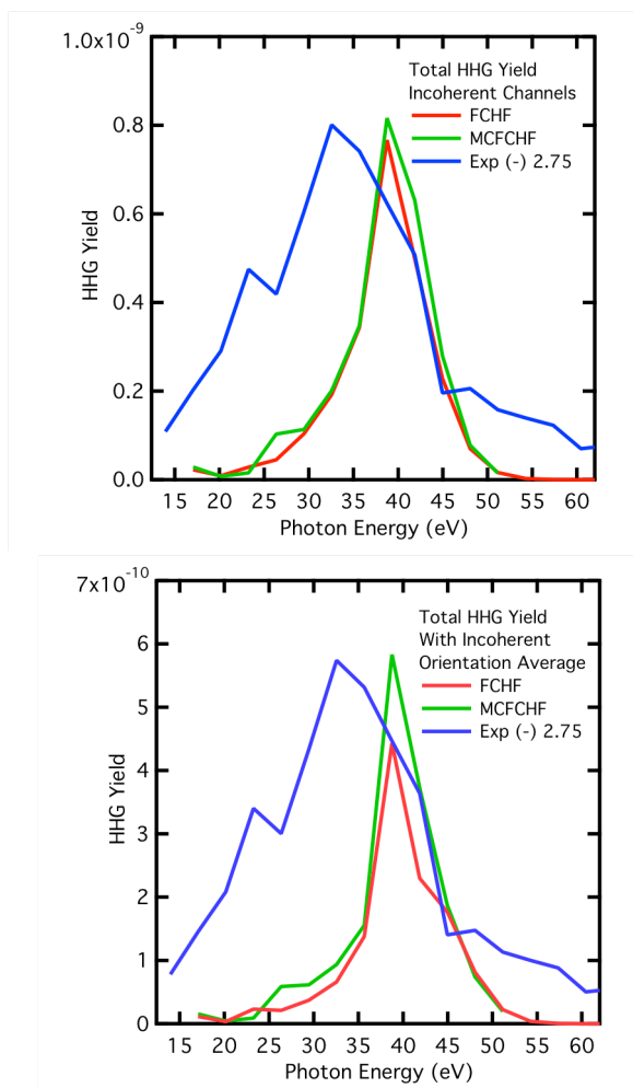
Figure 8: Top panel: The total of the QRS results from the three outermost valence orbitals of \text{SF}_6 shown in the middle column in Fig. 6. Bottom panel: The corresponding total of the incoherent orientation averages shown in the right panel in Fig. 6. The results in both panels are compared to the experimental HHG spectrum at 4.0 \times 10^{14} W/cm 2 with the focal point at (-)2.75 mm. The experimental scale is arbitrary and selected so that the maximum HHG yield is the same as the MCFCHF QRS results
