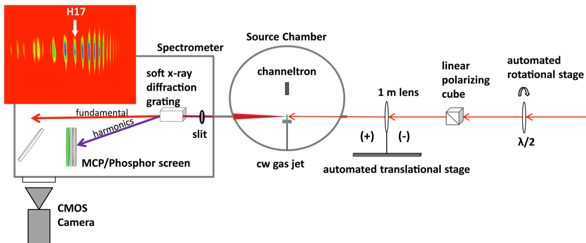
Figure 1: Block diagram of the experimental apparatus with a sample HHG image in the inset. The photon energy in the inset increases from left to right.
