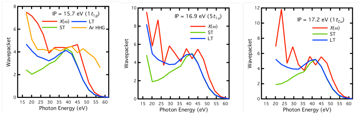
Figure 5. X^{\text{ref}}(\omega) for short (ST), long (LT) and for the full SFA integration. For HHG generation from the 1t_{1g} (HOMO), the wave packet generated from the experimental Ar HHG with the focus at (-) 2.75 mm and an intensity of 2.5 \times 10^{14} \text{ W/cm}^2 using Eq. (12) is also given.
