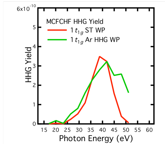
Figure 7. Comparison of QRS 1t_{1g} (HOMO) yield from the short trajectory wave packet calculation and using the experimental wave packet constructed from Ar HHG data using Eq. (12).
