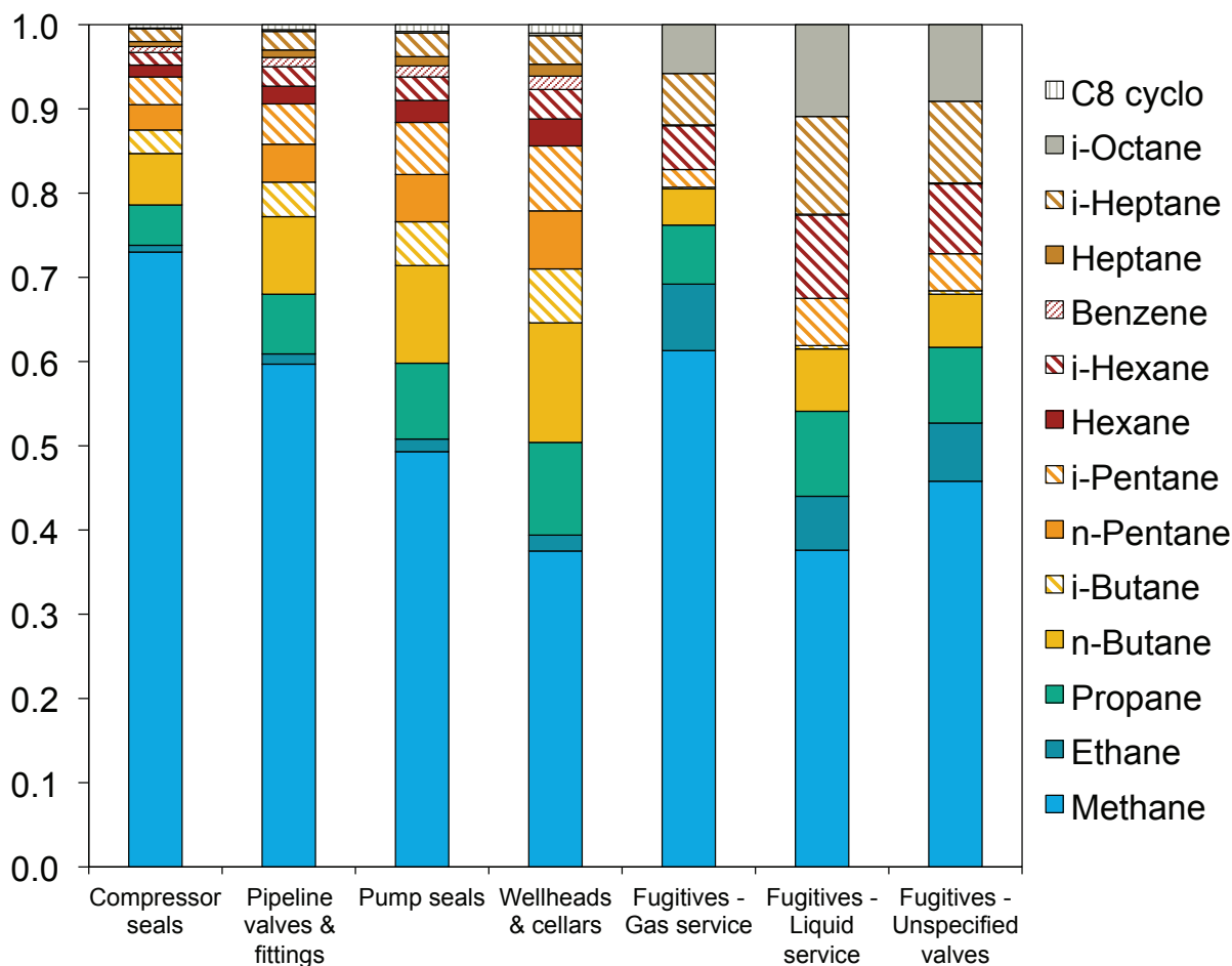
Figure 3.3-6. Stationary source speciation of TOG fugitive oil and gas production sources. Source: (CARB, 2014i)
