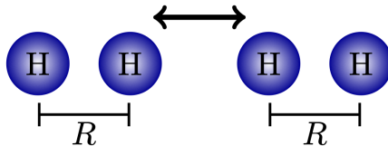
Figure 5.11: Schematic depiction of the dissociation process of (\text{H}_2)_2 in \text{D}_{\infty h} configuration.
