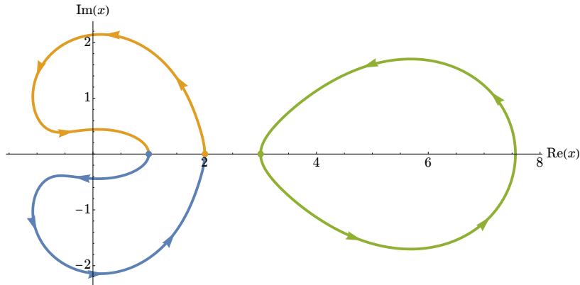
Figure 5.1: The paths of the roots of x^3 - 6x^2 + 11\gamma(\tau)x - 6 along \gamma : [0, 1] \rightarrow \mathbb{C}, \tau \mapsto e^{i2\pi\tau} .
