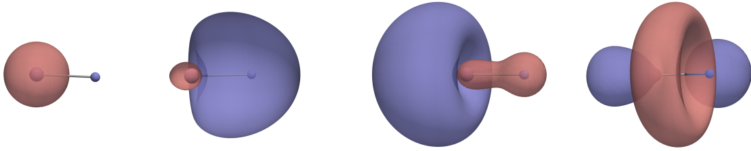
Figure 1.6: Iso-surfaces for \pm 0.04 of four molecular orbitals of lithium hydride.
