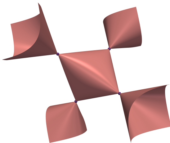
Figure 1.1: Affine Cayley cubic surface with the four singular points marked.
