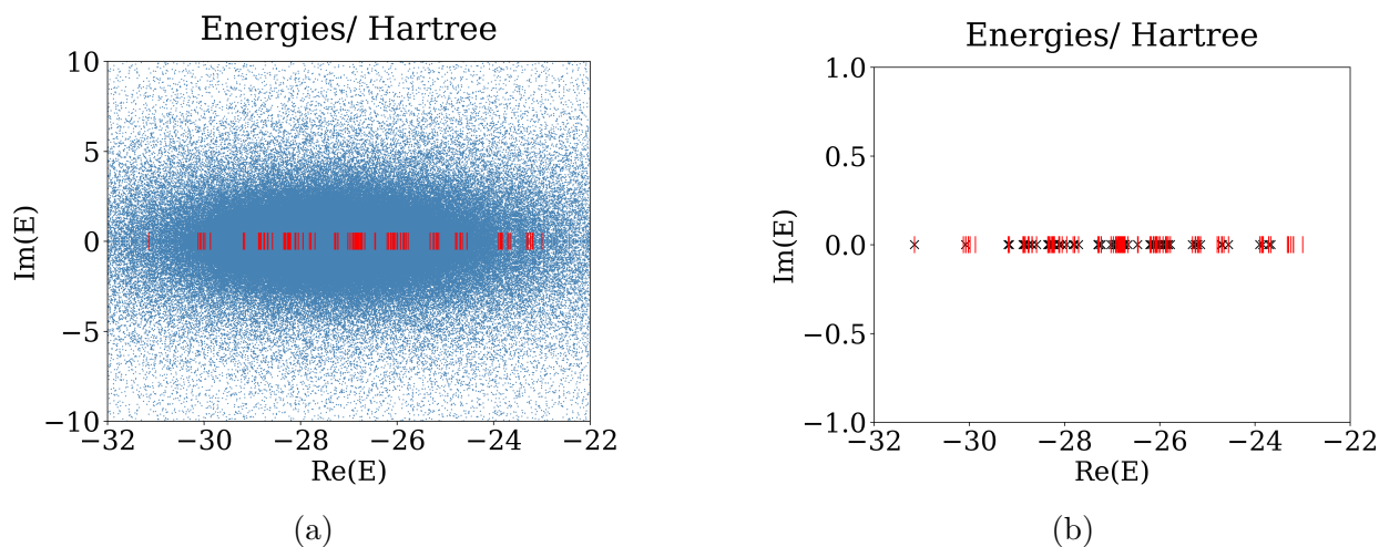
Figure 9.4: \text{H}_2\text{O} dissociation in a minimal basis ( k = 4 , m = 6 ): comparison of RCCD energies with the exact eigenvalues. (a) All RCCD energies compared to the exact spectrum. (b) RCCD energies lying near an eigenvalue (physically relevant).
