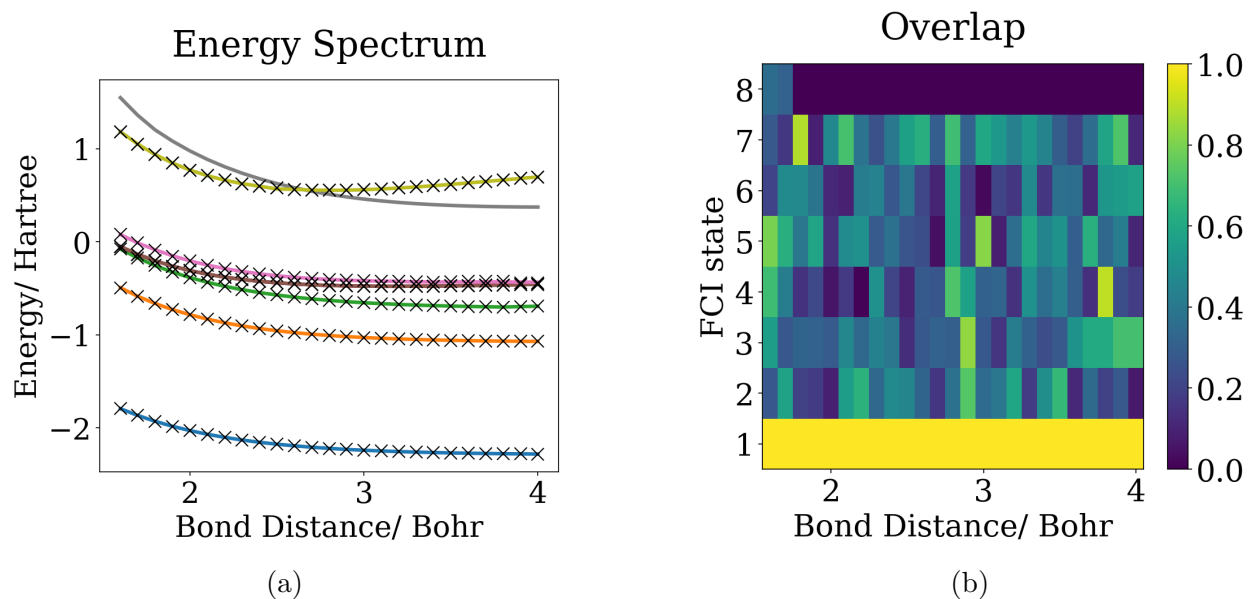
Figure 5.10: (a) PECs of (\text{H}_2)_2 in D_{2h} symmetry that are accurately described by CCD energies. (b) Overlap of the CCD states with the corresponding eigenstate.
