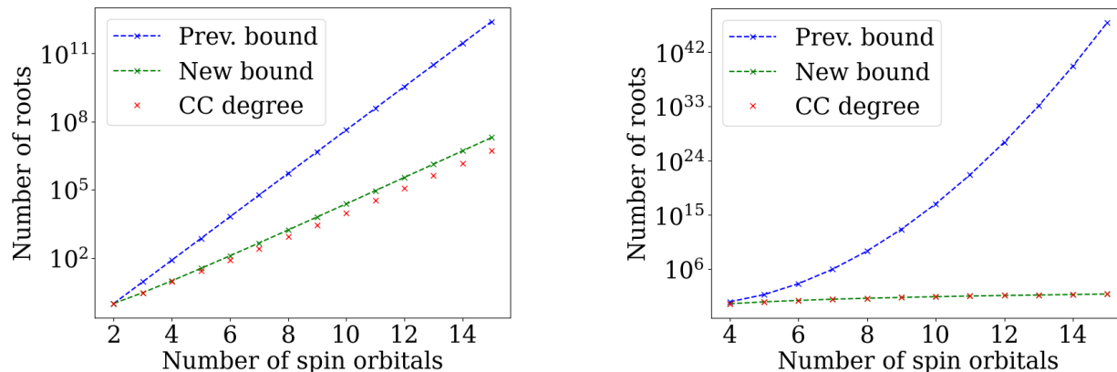
Figure 5.4: Bounds to the number of solutions for CCS (left panel) and CCD (right panel).
