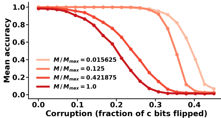
Figure 2.8: Factoring a corrupted \mathbf{c} . For M well below capacity (lighter curves above) one can sustain heavy corruption to \mathbf{c} and still find the correct factorization.
