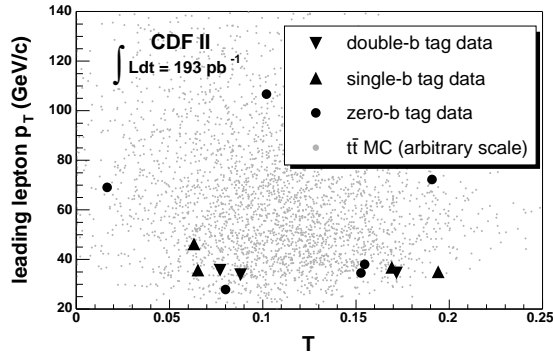
FIG. 2: Top dilepton events in (p_T^\ell, T) plane with b-tagging information.
