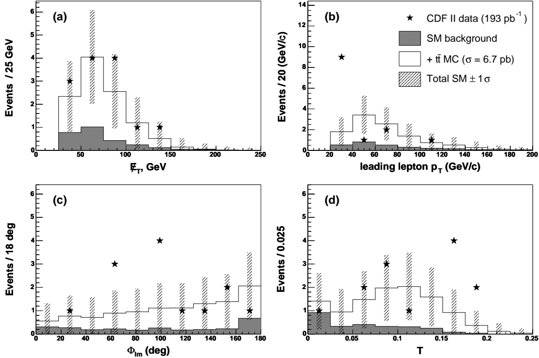
FIG. 1: \cancel{E}_T , leading lepton p_T , \Phi_{\ell m} , and T distributions for the top dilepton sample. The hatched regions represent the Poisson uncertainty on the expectation in a given bin.
