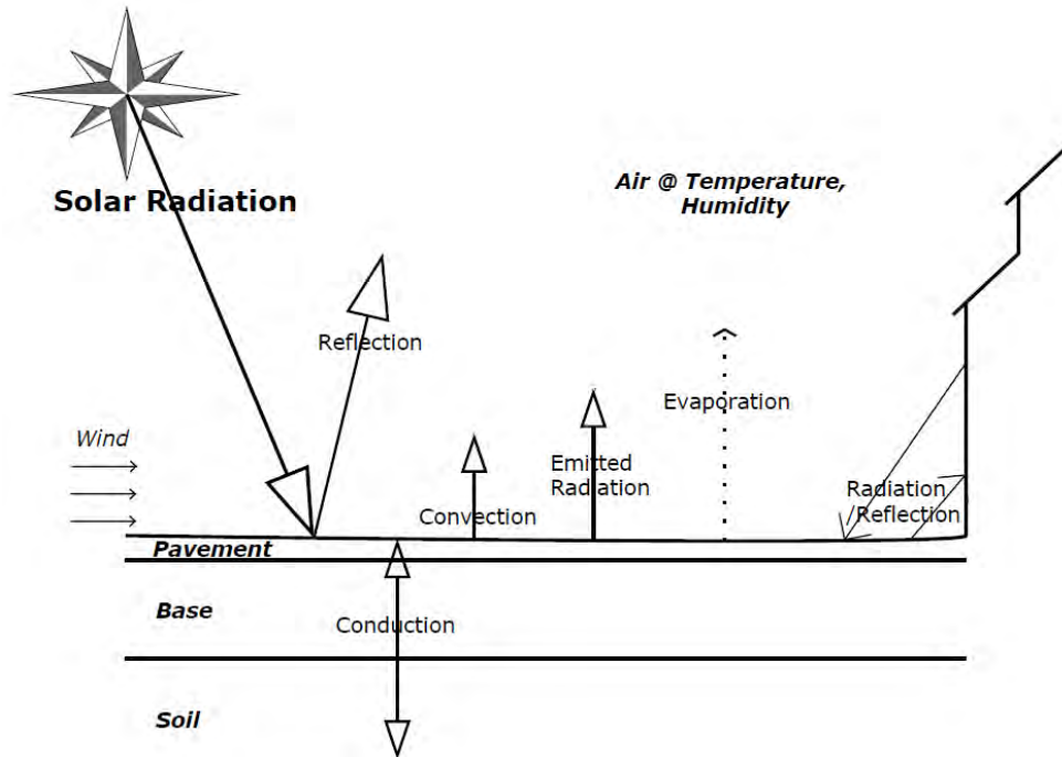
Figure 1.7. Energy balance on pavement surface.
