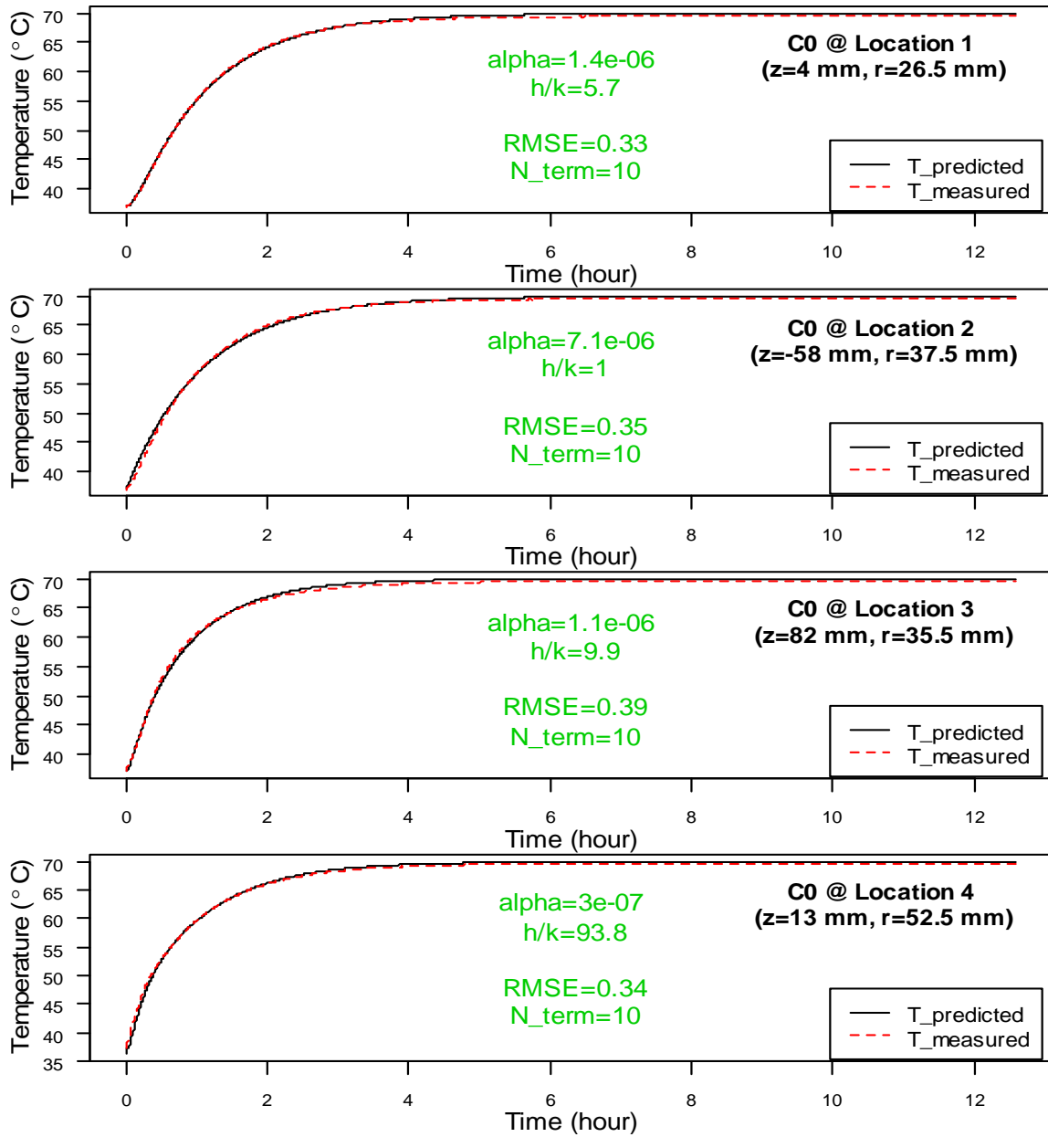
Figure 6.12. Predicted temperature with the optimized thermal properties compared with measured temperature: Concrete specimen C0. (unit: \alpha/a in \text{m}^2/\text{s} ; h/k in 1/\text{m} ; RMSE in ^{\circ}\text{C} .)
