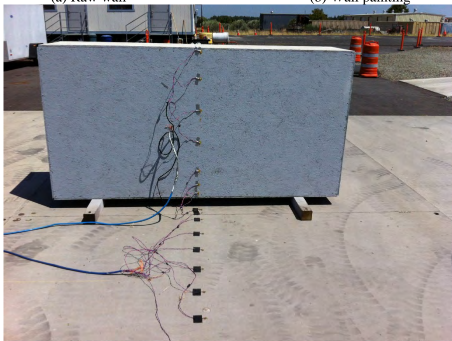
(c) Example test setup with temperature sensors
