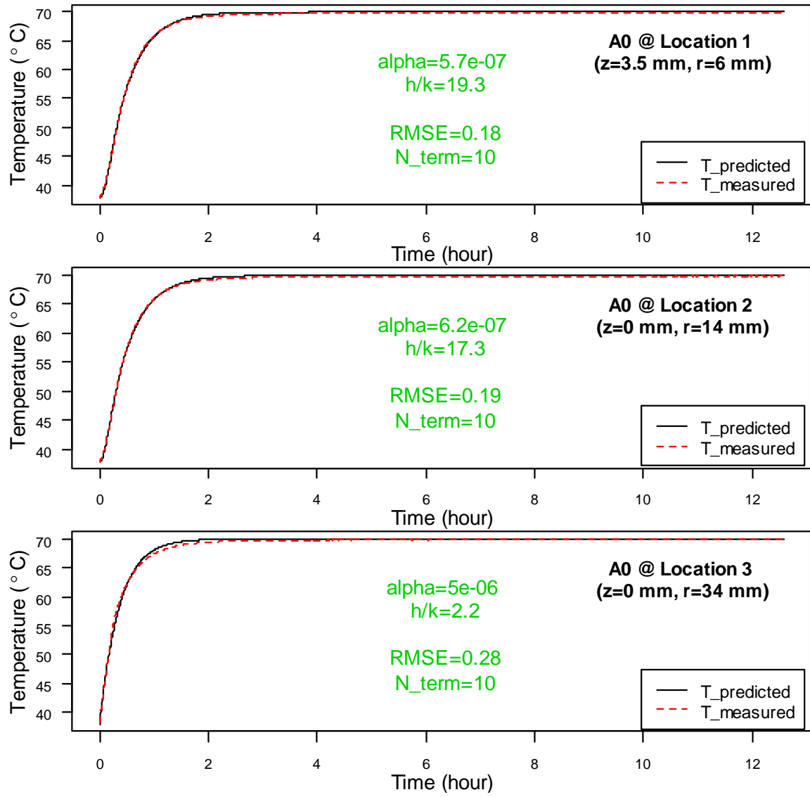
Figure 6.11. Predicted temperature with the optimized thermal properties compared with measured temperature: Asphalt specimen A0. (unit: \alpha/a in \text{m}^2/\text{s} ; h/k in 1/\text{m} ; RMSE in ^{\circ}\text{C} .)
