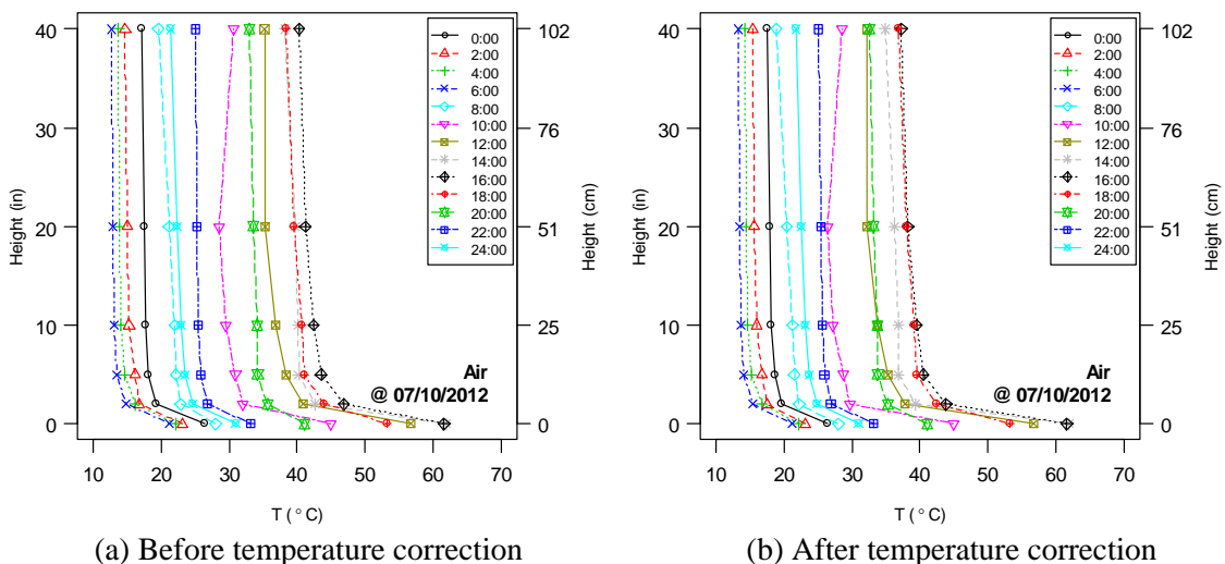
Figure 9.2. Example spatial profile of near-surface air temperature before and after correction (PA1).
