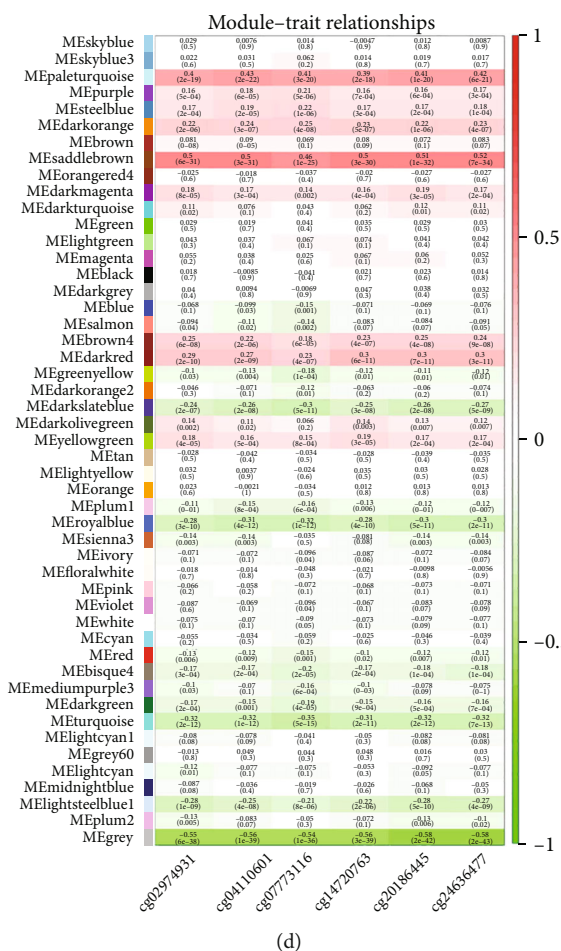
FIGURE 2: WGCNA-based identification of GMRGs. (a) Sample clustering of the dataset. The branches in the figure represent the samples and the vertical coordinate represents the height of the hierarchical clustering. The overall clustering of the combined data samples can be seen in the graph. (b) The distribution of scale-free soft threshold. The horizontal axis represents the weight parameter power value in both two graphs. The vertical axis of the left graph shows the scale-free fit index, i.e., signed R2 and the higher R2, the more the network will approximate the scale-free distribution. The vertical axis of the right graph represents the mean value of all gene adjacency functions in the corresponding gene module. (c) Module clustering tree diagram. Genes are classified into various modules by hierarchical clustering, with different colors representing different modules. The gray is for genes that cannot be classified in any module by default. (d) Heat map of correlations between modules and methylation sites. The vertical coordinate is for different modules, and the horizontal coordinate is for different sites. Each square indicates the correlation coefficient and significant P value for one module and one site. Red is for positive correlation, and green is for negative correlation. As the correlation level increases, the color becomes darker.
