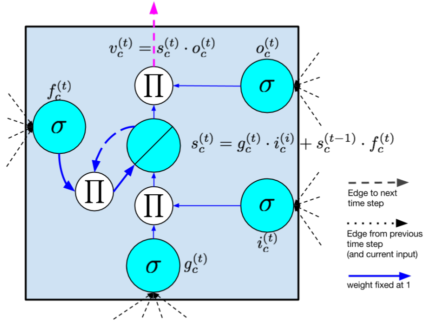
Figure 2.8: LSTM memory cell with forget gate as described by Felix Gers et al. in [GSC00].
