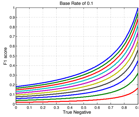
Figure 5.5: F1 score for fixed base rate and number fn of false negatives. F1 offers increasing marginal returns as a function of tn . Each line is a fixed value of fn .
