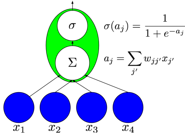
Figure 2.1: An artificial neuron computes a nonlinear function of a weighted sum of its inputs.
