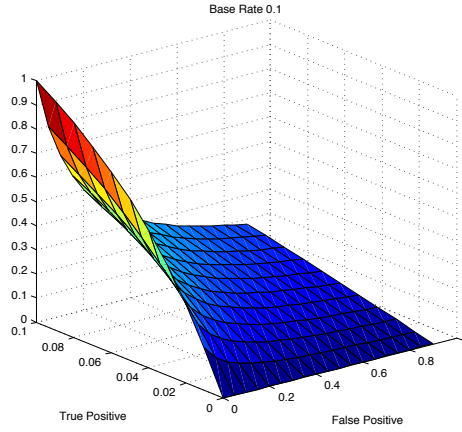
Figure 5.4: Given a fixed base rate, the F1 measure is a nonlinear function with two degrees of freedom.
