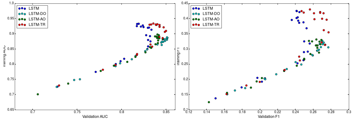
(c) AUC training vs. validation
