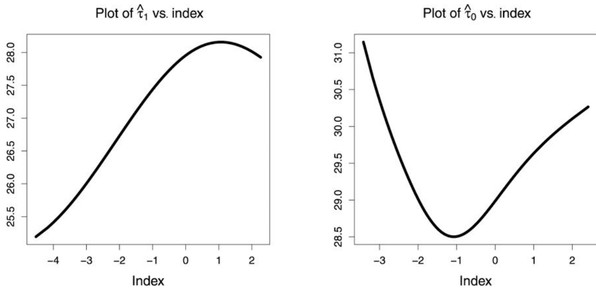
FIG. 3. The plots of \hat{\tau}_1 for the smoking group and \hat{\tau}_0 for the nonsmoking group, respectively, versus the estimated index value \hat{\mathbf{V}}^T X_i .
