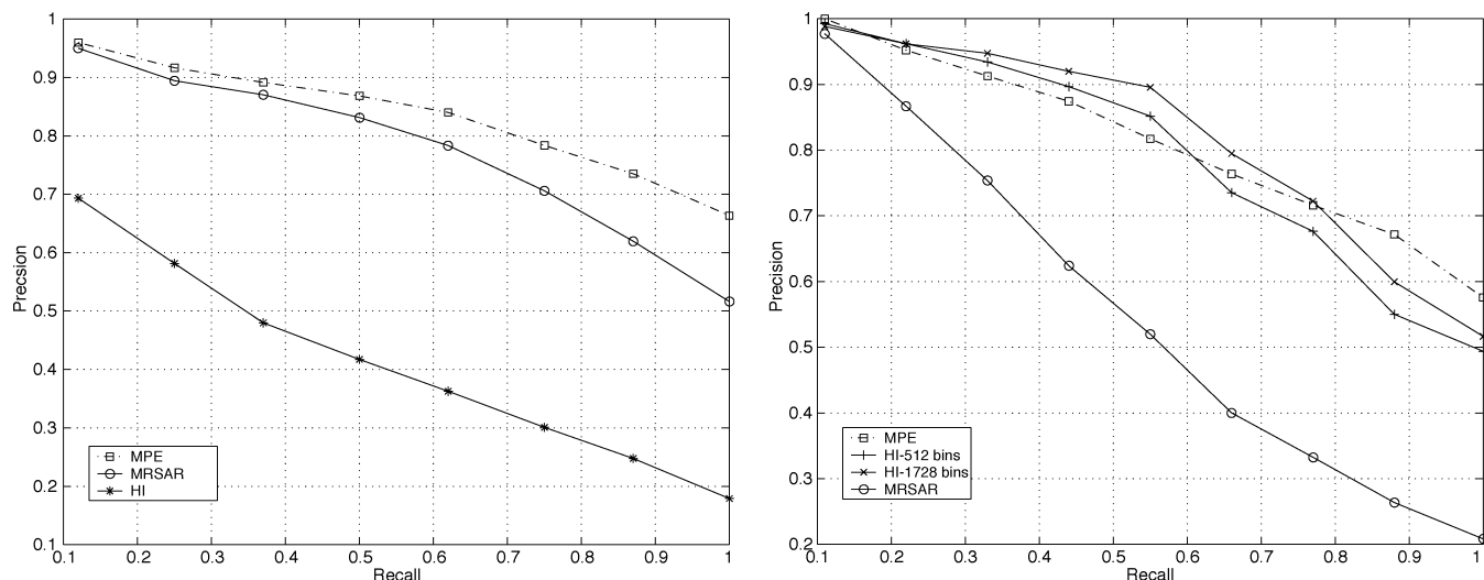
Fig. 6. PR measured for the MPE, MRSAR, and HI retrieval architectures. (Left) Curves from Brodatz, where the best results for HI (which are shown) were obtained with histograms of 192 bins. The features selected by MPE were the DCT set with 32 subspaces. (Right) Curves from Columbia where best HI results were obtained with histograms of 1728 bins. There was, however, a wide range of the number of bins where the performance was nearly constant, as illustrated by the second curve, which was obtained with histograms of 512 bins. The features selected by MPE were the DCT set with 48 subspaces.
