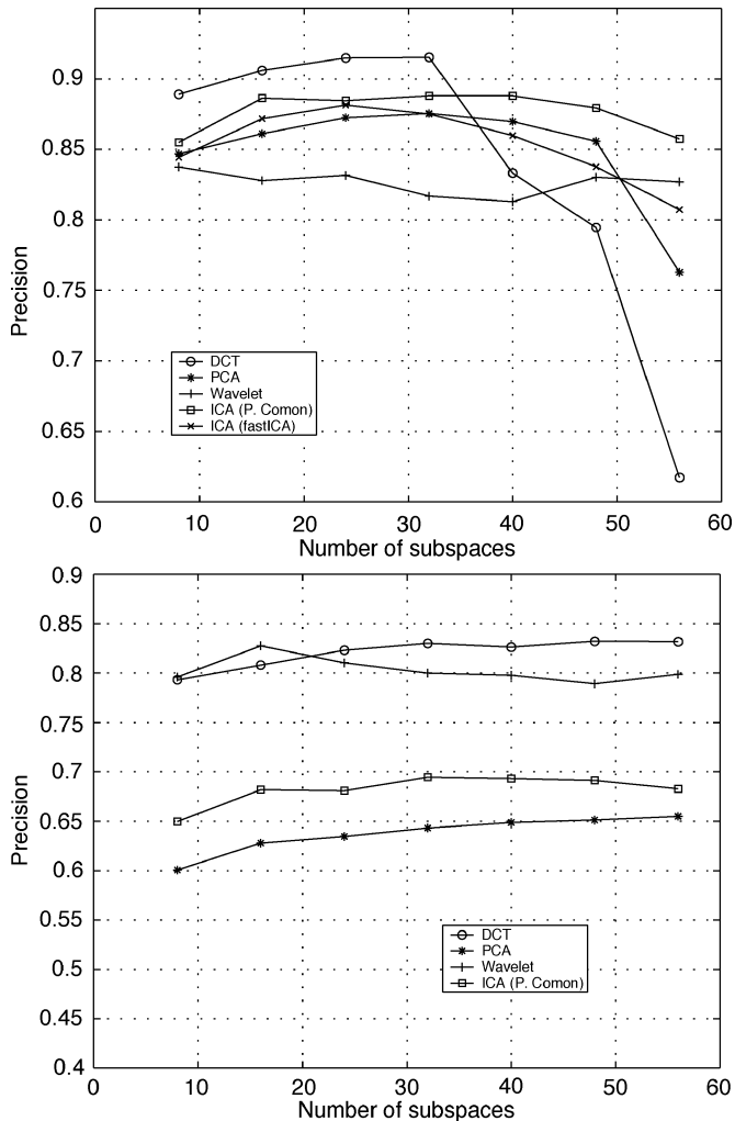
Fig. 5. (Top) Precision, at 30% recall on Brodatz. (Bottom) Precision, at 10% recall, on Corel.
