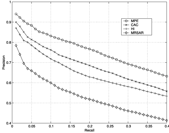
Fig. 8. PR on Corel for MRSAR, HI (512 bin histograms), color correlogram (CAC), and MPE retrieval. The features selected by MPE were the DCT set with 46 subspaces.
