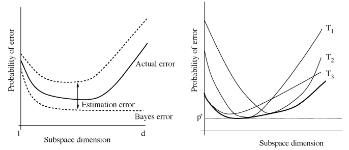
Fig. 1. (Left) Upper bound, lower bound, and probability of error as a function of subspace dimension. (Right) Curves of probability of error associated with three feature transformations. The convex hull is shown in dark, and its minimum value is p^* .
