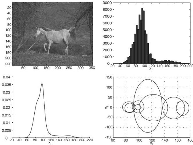
Fig. 3. (Top left) Image from the Corel database, (top right) its histogram, (bottom left) projection of the corresponding 64-dimensional embedded mixture onto the DC subspace, and (bottom right) projection onto the subspace of the two lower frequency coefficients. The embedded mixture describes the probability density of the discrete cosine transform coefficients derived from a collection of 8 \times 8 blocks extracted from the image.
