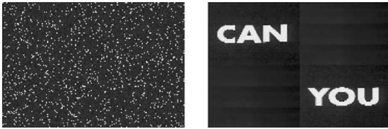
Fig. 4. Two images that, although visually very dissimilar, have the same color histogram.
