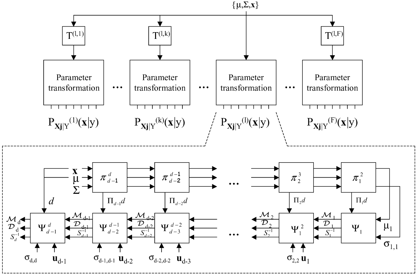
Fig. 2. Recursive algorithm for 1) propagating the parameters \{\mu, \Sigma\} of a mixture component in a reference space \mathcal{X}^{(l)} to all other features subspaces associated with T and 2) computing the components \mathcal{D}_j and \mathcal{M}_j of the similarity function on all feature subspaces. \Psi_{j-1}^j is the mapping that implements (23)–(27).
