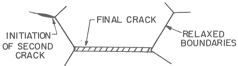
(c) FINAL FACET SIZED CRACK PRODUCED BY SLIDING RELAXATION
