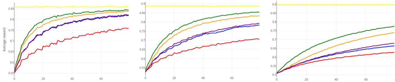
Figure 1: Performance of different agent types over 80 learning trials (x-axis), with N = 10, 25 , and 100 actions. The color key is as follows: yellow=Omniscient, orange=Softmax, red=Softmin, blue=Infomax, green=UCB, purple=Random.
