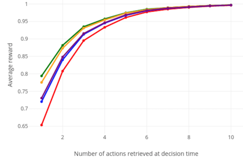
Figure 5: Uniform distribution on success probability means. R actions retrieved at decision time.
