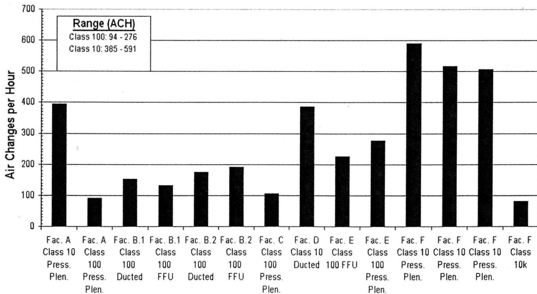
Figure 7. Air-change rate comparison.
