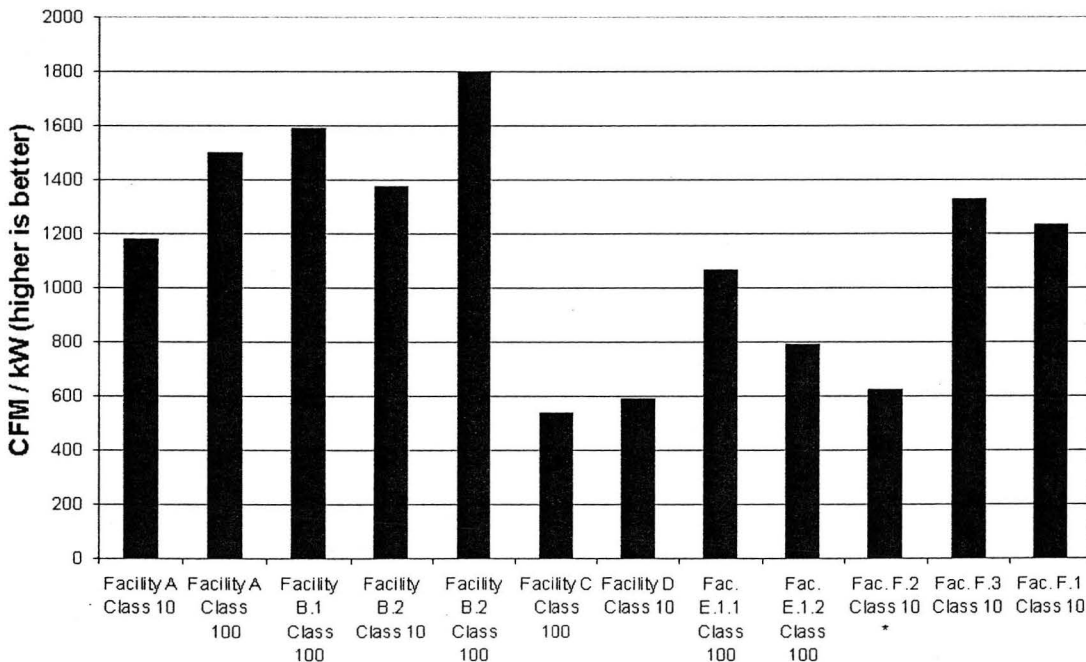
Figure 8. Make-up air comparison.
