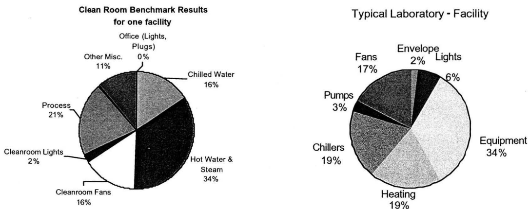
Figure 4. Energy end use.
