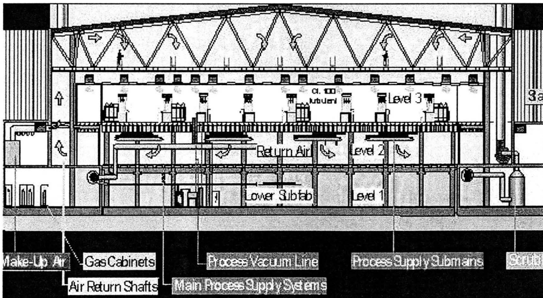
Figure 5. Semiconductor manufacturing facility.
