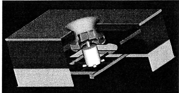
Figure 3. Fan-filter unit schematic.
