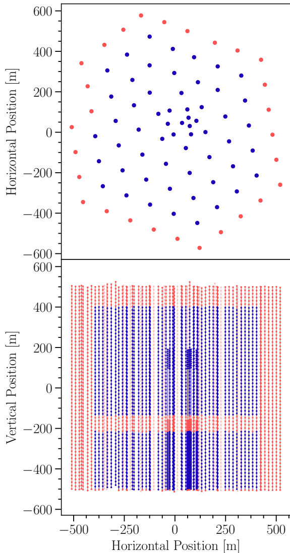
FIG. II.1. HESE veto. Diagram of the IceCube detector indicating veto DOMs. Top panel: an overhead view of the IceCube detector. Positions of strings with only veto DOMs are shown in red, while those with at least one non-veto DOM are shown in blue. Bottom panel: a side view of the IceCube detector strings and DOMs. Veto DOMs are indicated with red circles and non-veto DOMs with blue circles. Strings in front of or behind the region without veto DOMs are semi-transparent.
