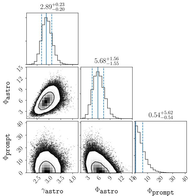
FIG. VI.6. Single power-law parameters posteriors. Diagonal panels show the one-dimensional posterior distribution of the parameters (joint distribution integrated over all other parameters), where the horizontal axis of the panel is the same as the horizontal axis at the bottom of the column, and the vertical axis of the panel is the probability density in an arbitrary scale. The solid blue lines denote the MAP estimator for each parameter, and the dashed lines denote the bounds of the one-dimensional 68.3 % HPD region; these numbers are also listed above the diagonal panels. Non-diagonal panels show the two-dimensional posterior distribution of the parameters, where the horizontal and vertical axes of the panel correspond to the horizontal axis at the bottom of the column and the vertical axis at the far left of the row, respectively. The innermost contours show the two-dimensional 68.3 % HPD region, and the outermost contours show the 95.4 % HPD region. The grayscale of the histogram within the contours shows the probability density in an arbitrary scale. The points outside the contours show individual points from the MCMC.
