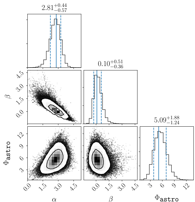
FIG. VI.10. Log-parabola astrophysical model parameters posterior distribution. Results derived from the posterior distribution of the model are shown in the same style as Fig. VI.6. The figure shows the one- and two-dimensional posterior distributions for the astrophysical flux normalization, \Phi_{\text{astro}} ; the spectral index at 100 TeV, \alpha ; and the change in spectral index, \beta . The diagonal panels show the one-dimensional posterior with the parameter MAP estimation and 68.3% HPD region indicated, while the non-diagonal panels show the two-dimensional posterior with 68.3% and 95.4% regions indicated. As we can see from the posterior distribution, \beta is compatible with zero which implies that an unbroken power law is a good fit to the data under these model constraints.
