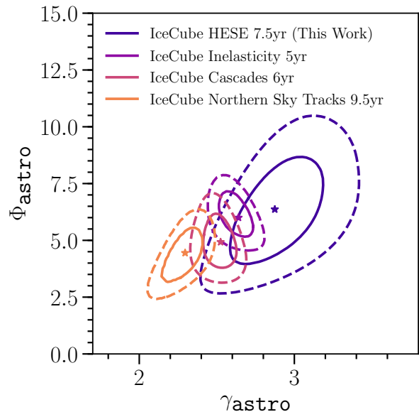
FIG. VI.3. Comparison of single power-law parameters from different analyses. Assuming an unbroken single power-law model for the astrophysical neutrino flux, results from different IceCube samples are shown. The horizontal axis is the spectral index of the model and the vertical axis is six-neutrino flux normalization at 100 TeV given as a dimensionless multiplicative factor relative to 10^{-18} \text{ GeV}^{-1} \text{ sr}^{-1} \text{ s}^{-1} \text{ cm}^{-2} . The stars denote the different best-fit points, solid contours show the 68.3% confidence region using the asymptotic approximation given by Wilks' theorem, and dashed contours show the 95.4% confidence regions. Blue represents results from this work, while the purple shows results from IceCube's 5yr inelasticity measurement [167], salmon shows results from IceCube's 6yr cascade sample [63], and orange shows IceCube's 9.5yr Northern track sample preliminary result [94]. The differing preferred regions of parameter space for the astrophysical flux between the samples suggest a level of discrepancy, however a small region of parameter space is compatible with all samples at the 95.4% level. Many checks have been performed for possible explanations of the discrepancy without definitive conclusions.
