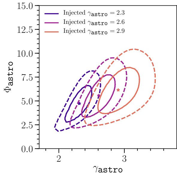
FIG. VI.5. Astrophysical parameter sensitivity to injected spectra. The three colors from blue to salmon show the expected astrophysical parameter 68.3% (solid lines) and 95.4% (dashed lines) uncertainty for three injected astrophysical spectra \gamma_{\text{astro}} \in \{2.3, 2.6, 2.9\} . In each of these cases the expected number of events for 7.5 years of lifetime is injected as data using nominal values for nuisance parameters and holding the number of injected astrophysical events to be equal between the spectra. As expected, the spectral index uncertainty grows with softer spectra from \sim 0.14 to \sim 0.21 when changing \gamma_{\text{astro}} from 2.3 to 2.9.
