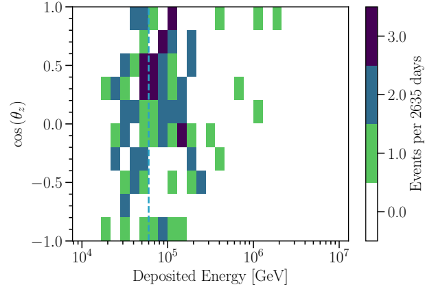
FIG. III.4. HESE events observed in 7.5 years. Histogram of the observed events as a function of their inferred deposited energy and cosine of the reconstructed zenith angle. The dashed line indicates the low-energy threshold of 60 TeV.
