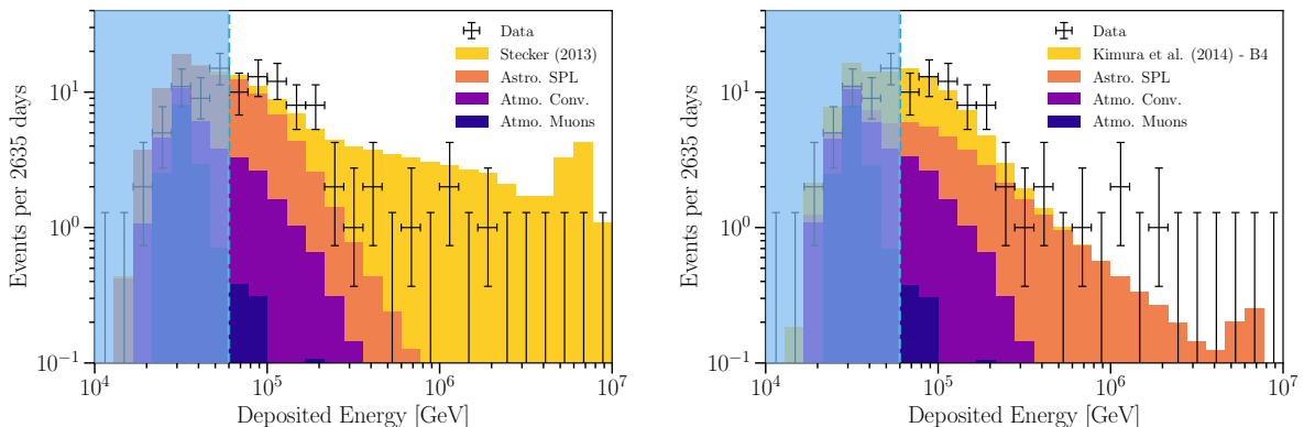
FIG. VI.14. Source-specific model energy distributions. Different panels show the predicted energy distribution compare to the data for a subset of the models considered in Table VI.3. In the cases shown above there are two astrophysical components: a specific source model and an additional single power-law component. All the components are shown as a stacked histogram at the best-fit value of the components normalizations. Left: The Stecker [197] model is shown as an example of a case where the Bayes factor assuming equally likely alternatives indicates significant preference for the single power-law model over the two component scenario. Right: The Kimura et al. (B4) [199] model is shown as an example of a case where an additional single power law is needed to explain the distribution of events.
