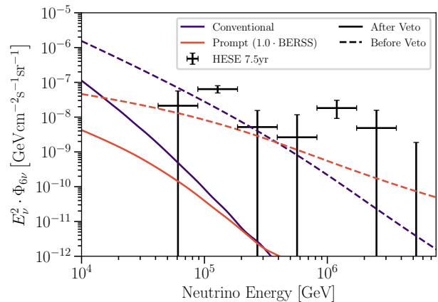
FIG. IV.5. All-sky average astrophysical neutrino flux and atmospheric neutrino fluxes in the vertical direction compared at \cos\theta_z = 1 before and after the veto. The atmospheric neutrino fluxes considered in this analysis are shown as dashed lines. The solid lines show the product of the atmospheric flux with the passing fraction averaged over depth at a zenith angle of 0^\circ . The frequentist segmented power-law fit of the astrophysical flux assumes isotropy, as described in Section VIA 5 is shown in black. This comparison demonstrates the effect of the veto in the down-going region, where it is strongest. The atmospheric flux suppression becomes weaker towards the horizon and is not present in the up-going region. The dashed lines labeled “before-veto” are equivalent to the up-going atmospheric fluxes, with or without the veto, neglecting Earth absorption effects.
