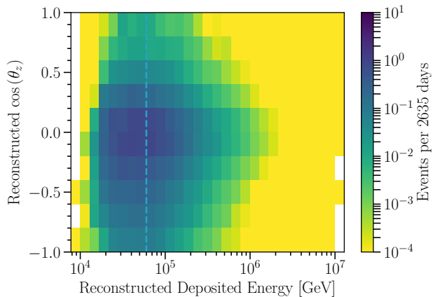
FIG. IV.3. Expected distribution of atmospheric neutrinos produced by pions and kaons in the sample. Distribution of neutrinos that pass the veto as a function of the deposited energy and the cosine of the zenith angle assuming nominal values for the nuisance parameters. The dashed line at 60 TeV marks the low energy cut of the analysis. Suppression in the down-going region is due to the veto. Suppression in the up-going region is due to absorption of neutrinos in the Earth.
