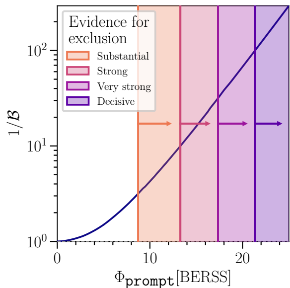
FIG. VI.13. Prompt neutrino normalization constraints. The horizontal axis shows the size of the prompt normalization with respect to the baseline BERSS model discussed in Section IV with passing fractions given in [120]. The vertical axis gives the reciprocal of the Bayes factor; decreasing Bayes factors imply a more disfavored prompt normalization. The shaded regions denote exclusions of the prompt normalization according to Jeffreys' scale from substantial to decisive.
