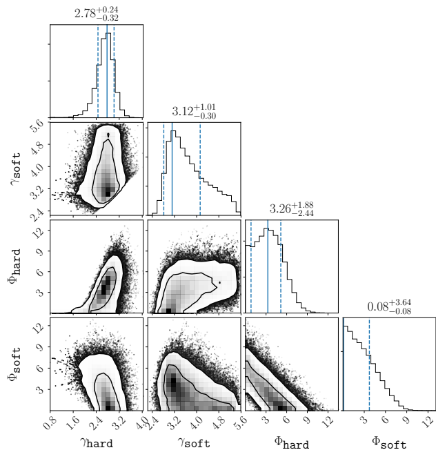
FIG. VI.7. Double power-law model hard/soft parameters posterior distribution. Results derived from the posterior distribution of the model are shown in the same style as Fig. VI.6. The figure shows the one- and two-dimensional posterior distributions for the parameters of the hard and soft components of the astrophysical neutrino flux. The diagonal panels show the one-dimensional posterior with the parameter MAP estimation and 68.3% HPD region indicated, while the non-diagonal panels show the two-dimensional posterior with 68.3% and 95.4% regions indicated.
