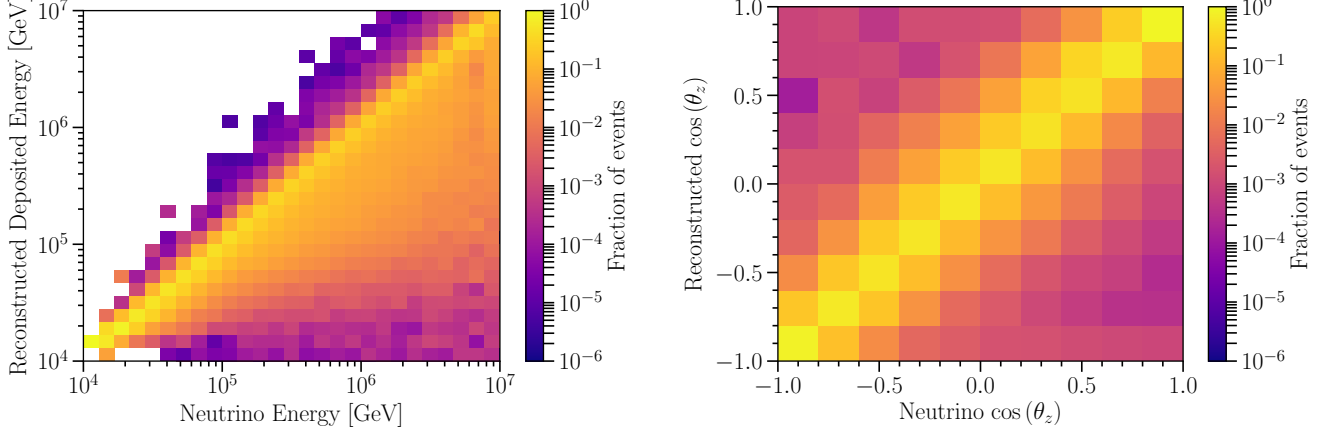
FIG. III.2. Distribution of expected reconstruction quantities as a function of true parameters. Transfer matrices, evaluated using simulation weighted to the single power-law best-fit parameters, are shown for all morphologies combined. The probability of a reconstructed deposited energy for a given neutrino energy (left) and the probability of a reconstructed cosine of the zenith angle for a particular cosine of the neutrino zenith angle (right) are shown. The matrices are column normalized. The asymmetry of the energy transfer matrix (left) is due to energy conservation, preventing large over fluctuations in reconstructed energy, and the wide range of visible energies possible for NC events which can lose large fractions of energy to the outgoing neutrino.
