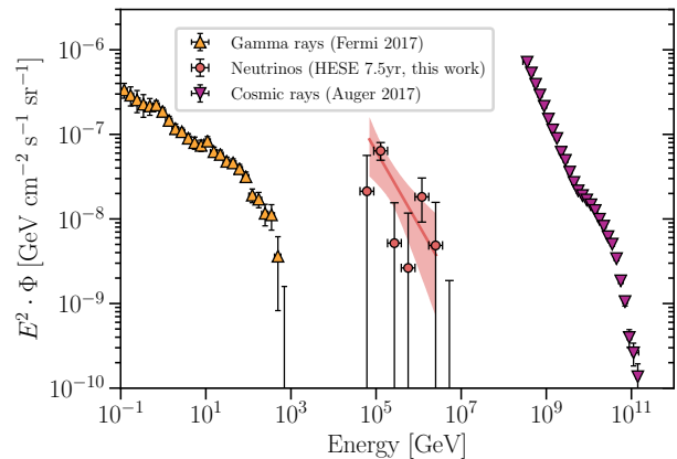
FIG. I.1. High-energy fluxes of gamma rays, neutrinos, and cosmic rays. The segmented power-law neutrino flux, described in Section VIA 5, obtained in the analysis described in this paper, is shown with red circles. The single power-law assumption, described in Section VIA 1, is shown with the light red region. The high-energy gamma-ray measurements by Fermi [73] are shown in orange, while the extremely-high-energy cosmic-ray measurements by the Pierre Auger Observatory [74] are shown as purple data points. The comparable energy content of these three fluxes is of particular interest in the investigation of cosmic-ray origin.
