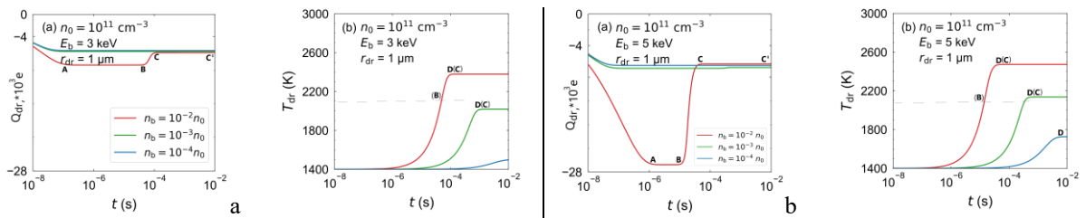
Fig. 1. Charge and temperature dynamics of a copper droplet with radius r_{dr}=1 \mu\text{m} ( n_0=10^{11} \text{ cm}^{-3} , note the use of a logarithmic time-axis): a) E_b=3\text{keV} , b) E_b=5\text{keV}
