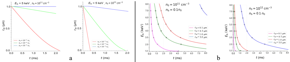
Fig. 2. a) Dynamic of the copper droplet's radius with initial size r_{dr} = 1 \text{ }\mu\text{m} : E_b = 5 \text{ keV} , n_0 = 10^{11} \text{ cm}^{-3} (on the left) 10^{12} \text{ cm}^{-3} (on the right); b) beam energy, that need for evaporation droplet with different size in giving time: n_0 = 10^{11} (left), n_0 = 10^{12} \text{ cm}^{-3} (right)
