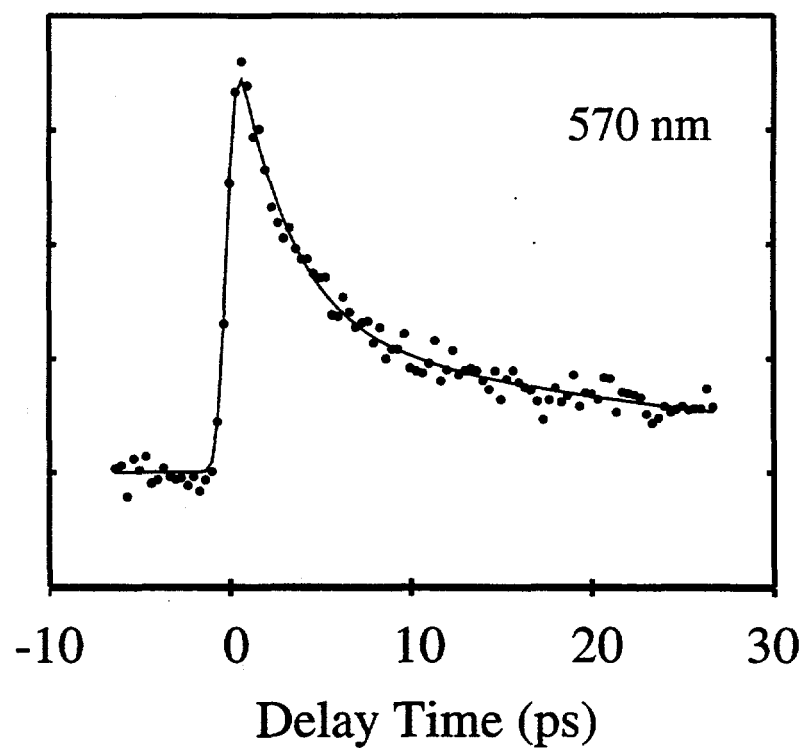
Figure 3.3 - Transient Absorption of \text{Cp}^*\text{Ir}(\text{CO})_2 in cyclohexane
