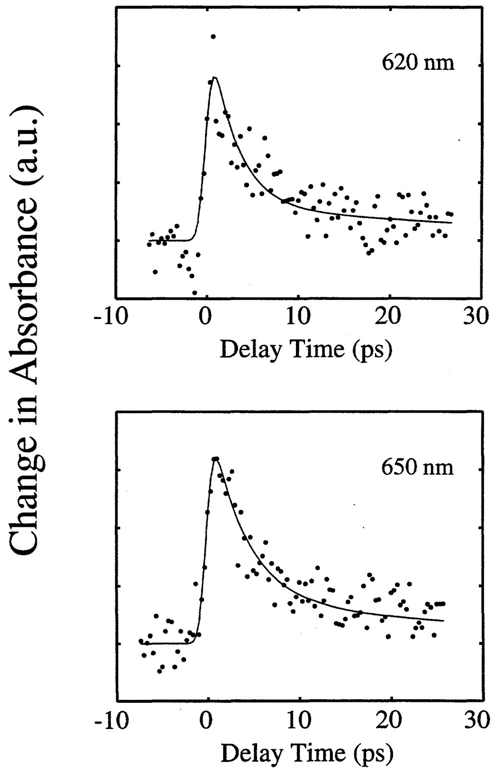
Figure 3.7 - Transient Absorption of \text{Cp}^*\text{Rh}(\text{CO})_2 in pentane
