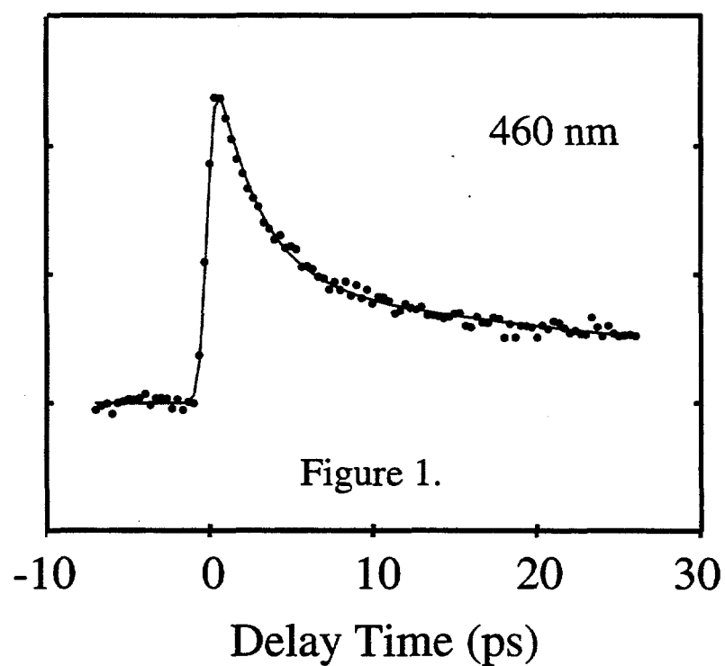
Figure 3.1 - Transient Absorption of \text{Cp}^*\text{Ir}(\text{CO})_2 in cyclohexane
