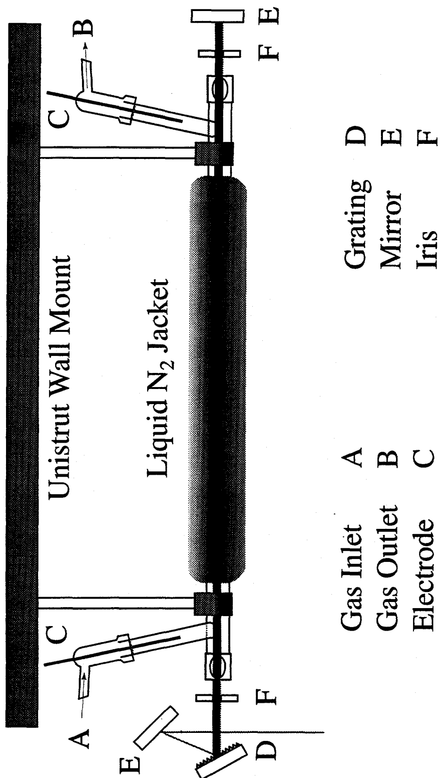
Figure 1.2 - The Layout of the CW Carbon Monoxide Laser
