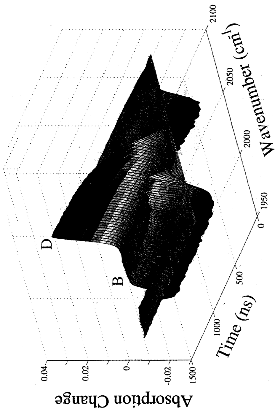
Figure 4.9 - Nanosecond Transient Absorption Spectrum of \text{Tp}^*\text{Rh}(\text{CO})_2 cyclohexane
