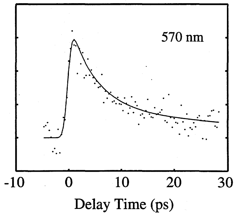
Figure 3.6 - Transient Absorption of \text{Cp}^*\text{Rh}(\text{CO})_2 in pentane
