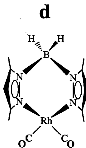
Figure 4.1 -C-H Activation reaction and structure of \text{Tp}^*\text{Rh}(\text{CO})_2
