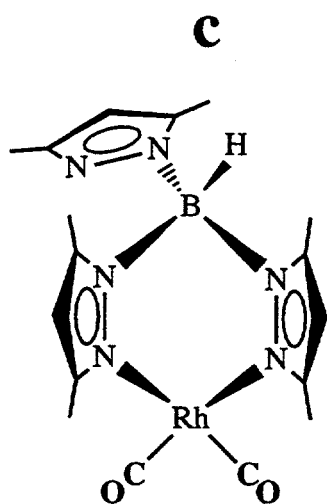
Figure 4.1 -C-H Activation reaction and structure of \text{Tp}^*\text{Rh}(\text{CO})_2
