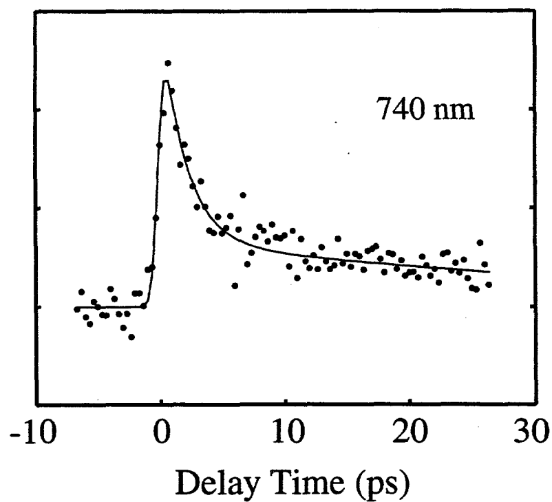
Figure 3.5 - Transient Absorption of \text{Cp}^*\text{Ir}(\text{CO})_2 in cyclohexane
