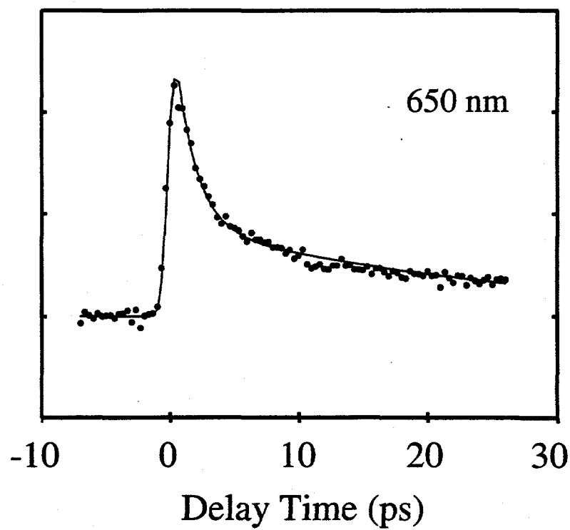
Figure 3.4 - Transient Absorption of \text{Cp}^*\text{Ir}(\text{CO})_2 in cyclohexane
