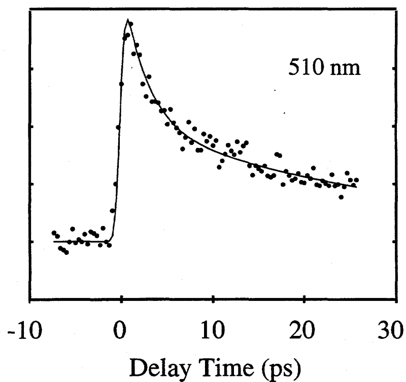
Figure 3.2 - Transient Absorption of \text{Cp}^*\text{Ir}(\text{CO})_2 in cyclohexane
