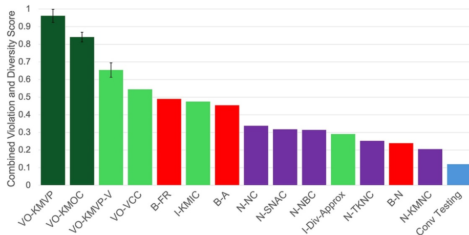
Figure 3. Fuzzing strategy comparison by combined violation and diversity score for retinal models. Each bar represents an average of normalized violations and normalized diversity score (with the linear normalization shown in figure 2), equally weighted. Each bar is the average of six tests, each with a different seed set, and error bars on the three best metrics show the standard error. Our metrics are shown in green, with our two best VO-KMVP and VO-KMOC highlighted in dark green. Neuron coverage metrics are shown in purple, and basic metrics in red. Conventional testing (model test set with no mutations) is shown in blue.
