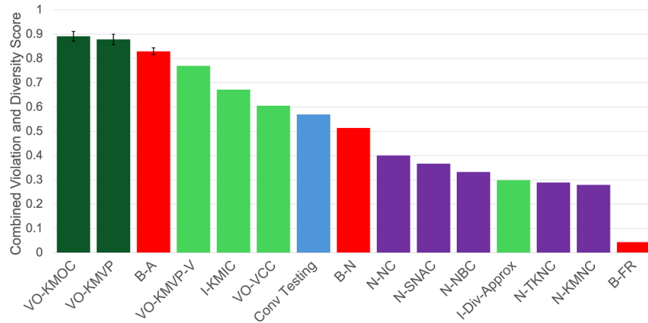
Figure 5. Fuzzing strategy comparison by combined violation and diversity score for cortical models. Each bar represents an average of normalized violations and normalized diversity score (with the linear normalization shown in figure 4), equally weighted. Each bar is the average of six tests, each with a different seed set, and error bars on the three best metrics show the standard error. Our metrics are shown in green, with our two best VO-KMVP and VO-KMOC highlighted in dark green. Neuron coverage metrics are shown in purple, and basic metrics in red. Conventional testing (model test set with no mutations) is shown in blue.
