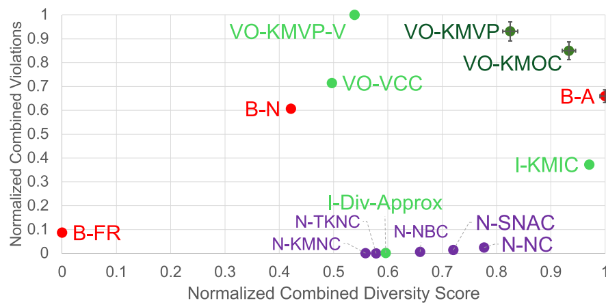
Figure 4. Fuzzing strategy comparison scatterplot for cortical models. Y-axis: number of violations found, normalized using linear normalization to a [0–1] range; x-axis: normalized combined diversity score (also using linear normalization to a [0–1] range). Each datapoint is the average of six tests, each with a different seed set, and error bars on the three best metrics show the standard error. Our metrics are shown in green, with our two best VO-KMVP and VO-KMOC highlighted in dark green. Neuron coverage metrics are shown in purple, and basic metrics in red.
