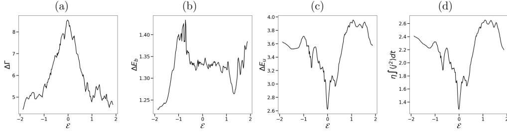
Figure 12: Accumulative diagnostics as a function of initial vortex eccentricity \varepsilon . The diagnostics are computed over 0 \leq t \leq 10 and show (a) the net circulation reduction \Delta\Gamma , (b) the net growth in magnetic energy \Delta E_b , (c) the net decline in kinetic energy \Delta E_u , and (d) the net magnetic dissipation \eta \int_0^{10} \langle j^2 \rangle dt . All simulations used the parameters \delta = 0.025 and \gamma = 1 .
