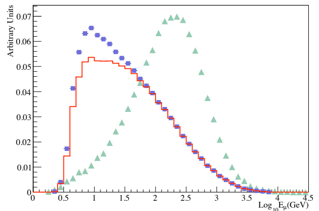
FIG. 1: The muon energy spectrum (given in \log_{10}(E_\mu) ) in the SNO detector from cosmic-ray muons (triangles) as predicted from MUSIC, and from neutrino-induced muons (boxes) created in the surrounding rock as predicted from the Bartol 3D Monte Carlo. The expected spectrum after oscillations is shown by the solid line. The distributions are not to scale.
