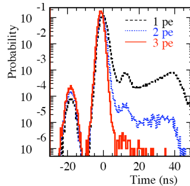
FIG. 2: The probability distribution of PMT firing times based on simulation for events with one (dashed), two (dotted), and three (solid) photons striking the photocathode.
