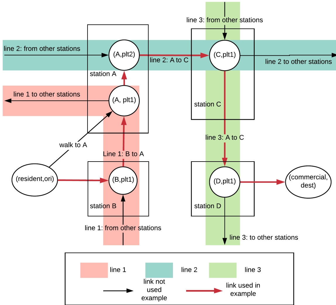
Figure 2. Physical network
