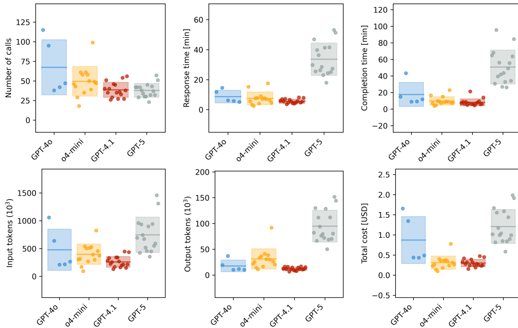
Figure 3: Comparison of four OpenAI models with the ML prompt across different high-level behavior metrics: number of calls, response time, completion time, input tokens, output tokens and total cost (see Appendix B for the exact definition of these quantities). Only successful runs are shown. The mean is marked with a line and the one standard deviation with a shaded box.
