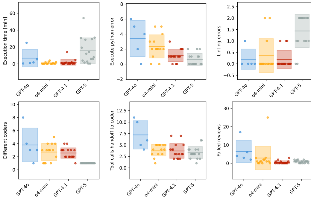
Figure 4: Comparison of four OpenAI models with the ML prompt across different metrics related to coding: execution time, execute python errors, lint errors, number of different coders used, tool calls handoff to coder and failed reviews (see Appendix B for the exact definition of these quantities). Only successful runs are shown. The mean is marked with a line and the one standard deviation with a shaded box.
