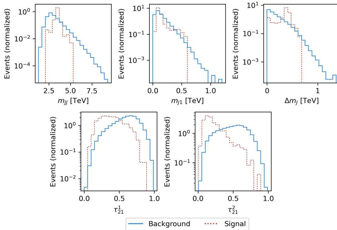
Figure 14: Normalized distributions of background (blue) and signal (red) for the following features in the full mass range LHC dataset: dijet invariant mass ( m_{JJ} ), the invariant mass of the lighter jet ( m_{J1} ), the difference between the invariant masses of the two jets ( \Delta m_J ), and the n-subjettiness ratios ( \tau_{21}^i ) for both jets.
