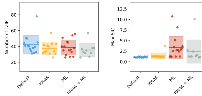
Figure 6: Comparison of the different prompt strategies using GPT-4.1, showing number of calls and max SIC. Only successful runs are shown. The mean is marked with a line and the one standard deviation with a shaded box.
