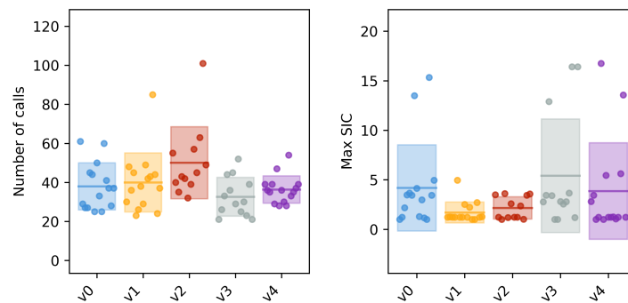
Figure 7: Comparison of the different prompt paraphrasings using GPT-4.1, showing the number of calls and the maximum SIC. Only successful runs are shown. The mean is marked with a line and the one standard deviation with a shaded box.
