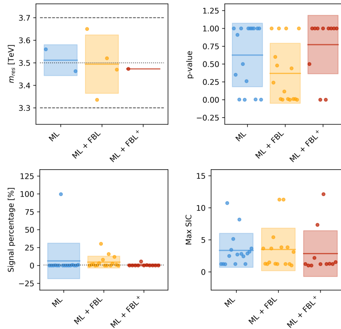
Figure 11: Comparison of the FBL prompts across metrics: m_{res} , p-value, signal percentage and max SIC using GPT-4.1. The mean is marked with a line and the one standard deviation with a shaded box. Note that since only one m_{res} value was reported with the ML+FBL + prompt, no standard deviation can be shown in that case.
