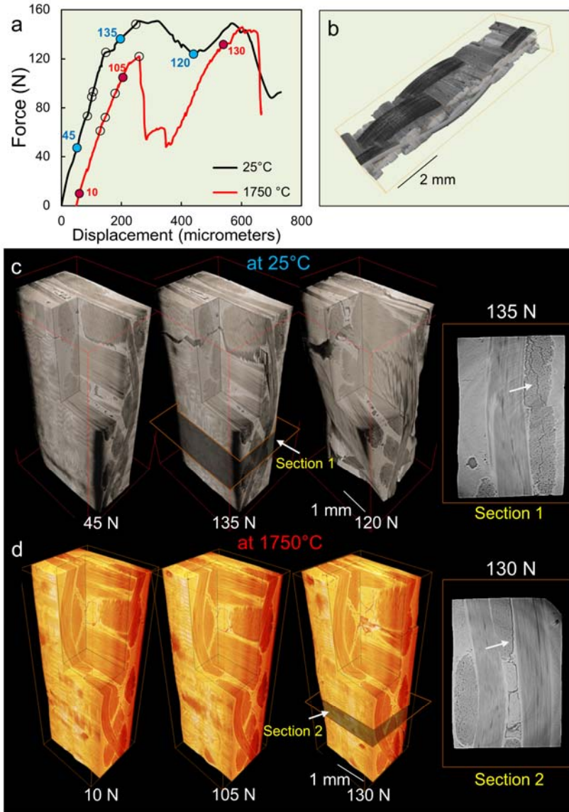
Figure 4. In situ tomography of C-SiC composite with textile-based carbon fiber reinforcements under tensile load at 25°C and 1750°C. (a) Force-displacement curves showing loads at which \mu -CT data were collected. Red curve offset by 60 \mu m for visual clarity. Hollow circles indicate acquired \mu -CT data at that load; blue and red solid circles indicate loads corresponding to images in (c) and (d) respectively. (b) \mu -CT image from composite plate after partial infiltration of SiC matrix illustrates the architecture of the woven fiber tows within the test samples. (c) & (d) \mu -CT images showing development of damage in specimens tested at room temperature (c) and at 1750°C (d). The higher magnification slices at the right, from sections 1 and 2, show different cracking mechanisms (indicated by arrows) in the later stages of failure: at room temperature, splitting cracks grow within the axial fiber tows; at high temperature, cracks grow along the boundary between the axial fiber tows and the matrix. Additionally, detailed animations of the complete sets of \mu -CT data from these two tests are included in the videos S3 and S4 in the Supplementary online information.
