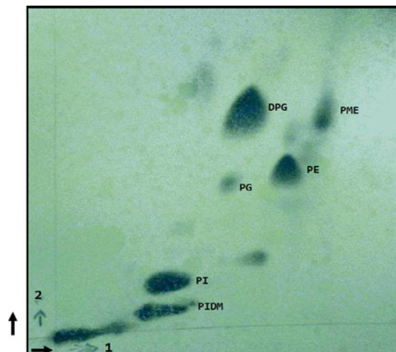
Fig. 4 Two-dimensional-chromatography of polar lipids of Salinispora pacifica CNR-114 T stained with molybdophosphoric acid spray (Sigma). Chloroform: methanol: water (32.5: 12.5 : 2.0 v/v) was used in the first direction and chloroform: acetic acid: methanol: water (40: 7.5: 6.2 v/v) in the second direction. DPG diphosphatidylglycerol, PE phosphatidylethanolamine, PG phosphatidylglycerol, PI phosphatidylinositol, PME phosphatidylmethylethanolamine, DM phosphatidylinositol dimannosides
