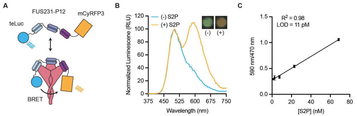
Fig 3. FUS231-P12 enables detection of SARS-CoV-2 S trimer through BRET.
