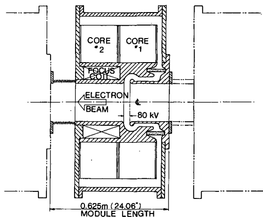
Fig. 3. Schematic of one of the 64 accelerator modules.
