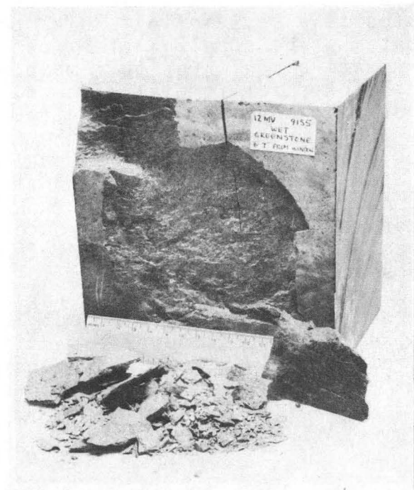
Fig. 1. Stress wave propagation. Fig. 2. Example one-shot spall.
