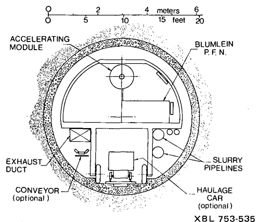
Fig. 4. Section at accelerator unit.
