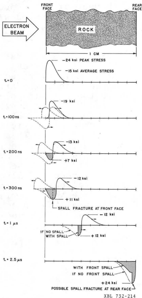
Fig. 1. Stress wave propagation. Fig. 2. Example one-shot spall.
