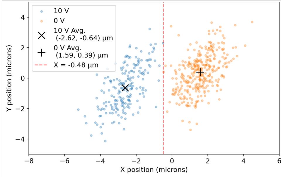
Figure 13. Laser centroid position when using discrete 10 V actuation of cell 19 of TAO Segment 3A at an \sim 1 s cycle. The mean laser deflection distance between the 0 V and 10 V states was 4.33 \mu\text{m} .
