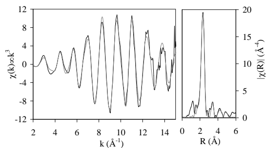
Figure 3. EXAFS spectrum and Fourier Transform of [\text{Ru}_p/\text{SiO}_2] . Data is black and fit is grey.
