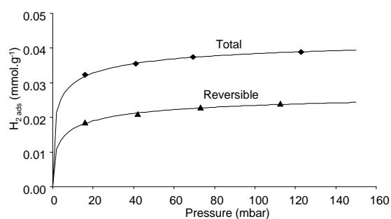
Figure 4. Hydrogen adsorption on [\text{Ru}_p/\text{SiO}_2] (sample 2). \blacklozenge Total adsorption. \blacktriangle Reversible adsorption. — Simulated Langmuir adsorption isotherms.
