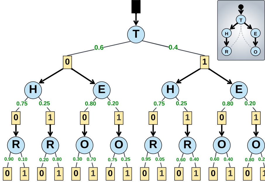
Figure 2.6: Example of an AND/OR search space for our runnin example model, guided by the pseudo tree from Section 2.1.4: Pseudo Trees. For simplicity, we abbreviate domain values of low or no instead with the value [0], and high or yes with [1]. We see that the search tree is more compact than that of the OR search tree in Figure 2.4.
