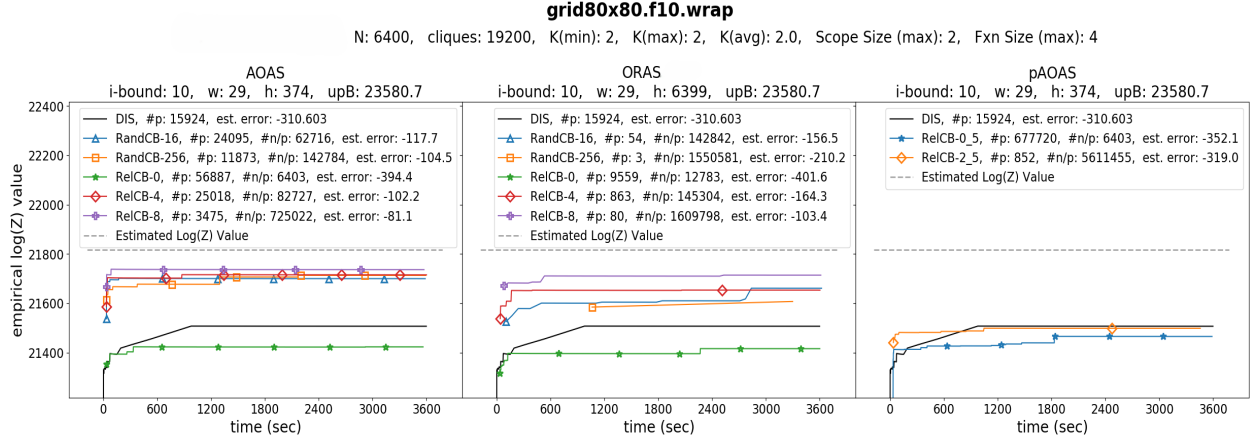
(a) Plots for a representative large Grid problem.
