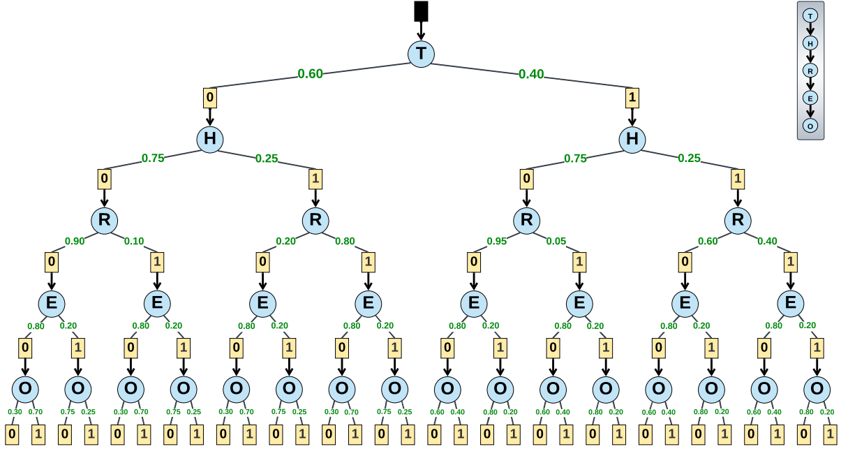
Figure 2.9: The OR search space from Figure 2.4 expressed explicitly as an AND/OR search space.
