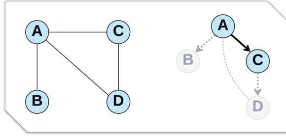
(a) Primal graph and truncated pseudo tree.
