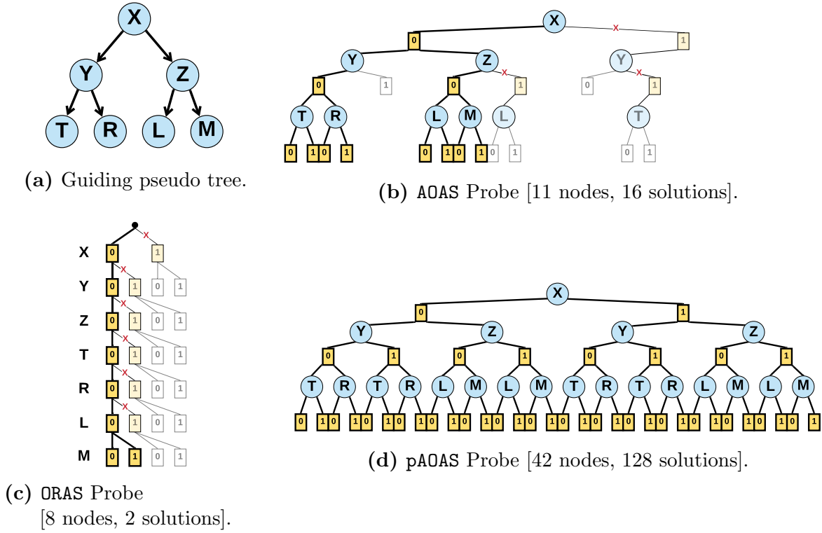
Figure 3.10: Contrasting scalability of various Abstraction Sampling schemes.
