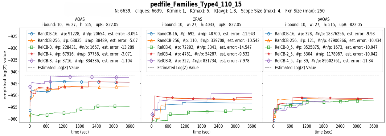
(b) Plots for a representative Linkage-Type4 problem. Note that DIS is omitted as it was unable to produce estimates for these problems.
