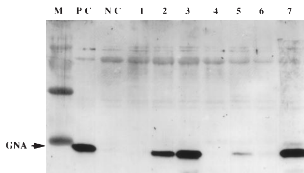
Fig. 4. Representative western blot analysis for GNA expression in R0 transgenic rice plants. Protein was extracted from young leaves and 20 µg was loaded in each lane. M, protein marker; PC, 100 ng purified GNA protein (positive control, 12 kDa); NC, untransformed plant (negative control); lanes 1–7, transgenic plant Nos. 7, 8, 9, 10, 11, 12 and 1 respectively. Plant Nos. 7 and 10 are negative for gna expression, plant Nos. 11 and 12 are weak expressers, plant No. 8 is a moderate expresser whereas plant Nos. 9 and 1 are high expressers
