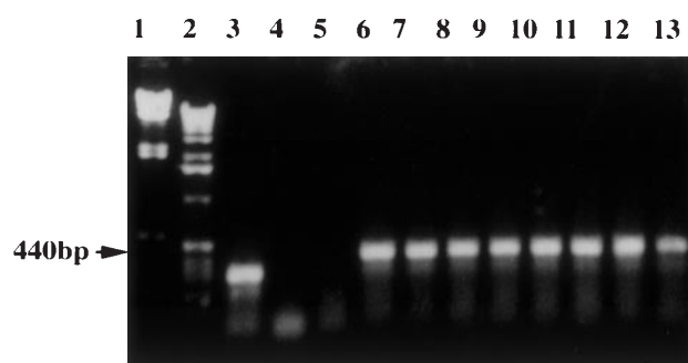
Fig. 5. Representative RT-PCR analysis for Xa21 transcription in R0 transgenic rice plants. Lane 1, size markers ( Hind III-digested λ DNA); lane 2, size markers (1-kbp DNA ladder); lane 3, positive control from Access RT-PCR System, producing a 323-bp band; lane 4, water (negative control); lane 5, untransformed plant (negative control); lanes 6–13, transgenic plants Nos. 1, 7, 8, 9, 10, 11, 12, and 13 respectively. The arrow indicates the expected RT-PCR product of the Xa21 mRNA (440 bp)
