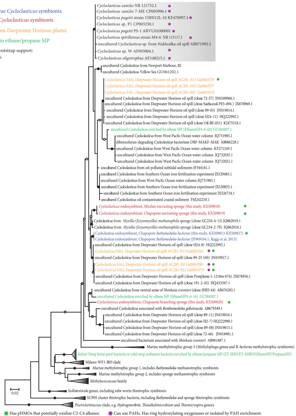
Figure 3. Phylogeny of Cycloclasticus 16S rRNA genes.
