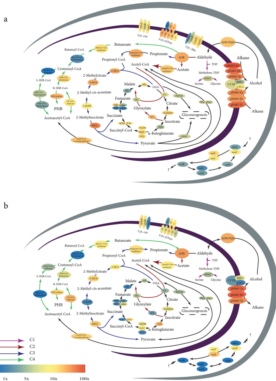
Figure 4. Reconstruction of central carbon and energy metabolic pathways in symbiotic Cycloclasticus .
