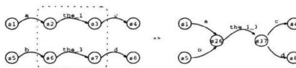
Terminal Merging in a Szilard DFA preserves the property one terminal appears on one arc only.
