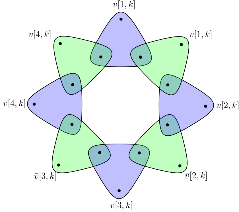
Figure 4.2: The ring structure for the embedding of 3SAT- B into 3DM-3. The ring shown corresponds to a variable u_i with d_i = 4 . An optimal matching in the ring corresponds to a truth value of for the variable u_i : the blue edges correspond to the value true while the green edges correspond to the value false .
