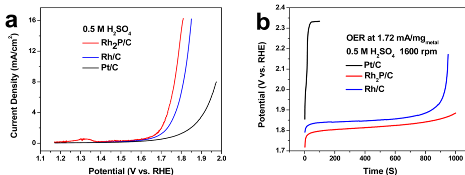
Figure 4. OER activity and stability in acid (0.5 M H 2 SO 4 ). (a) Polarization curves for Pt/C (3.7 \mu\text{g}_{\text{Pt}}/\text{cm}^2 ), Rh 2 P/C (3.7 \mu\text{g}_{\text{Rh}}/\text{cm}^2 ), and Rh/C (3.7 \mu\text{g}_{\text{Rh}}/\text{cm}^2 ) recorded at 20 mV/s. (b) Chronopotentiometry of the Rh 2 P/C, Rh/C, and Pt/C recorded at 1.72 mA/mg metal current density and room temperature while rotating at 1600 rpm. The potentials were converted to RHE and corrected for iR drop.
